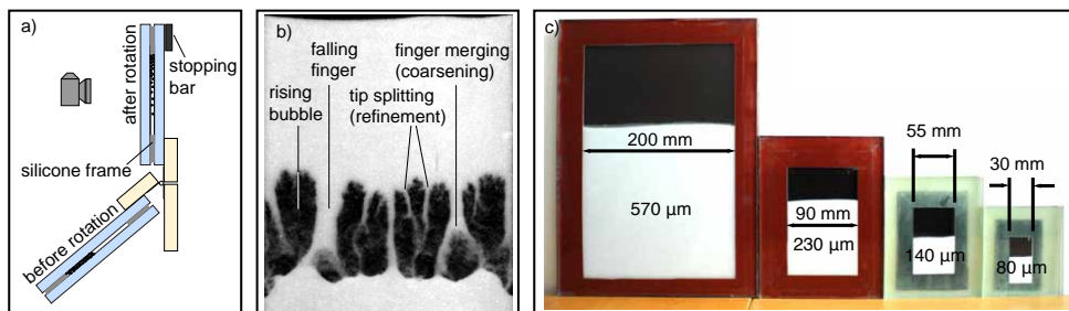
Fig. 1. (a) Experimental setup and principle, (b) typical granular Rayleigh-Taylor flow, where fingers of falling grains (white) form in the previously air-filled region (black) during an experiment, and (c) the experimental cells of different sizes with grains of proportional diameters.
