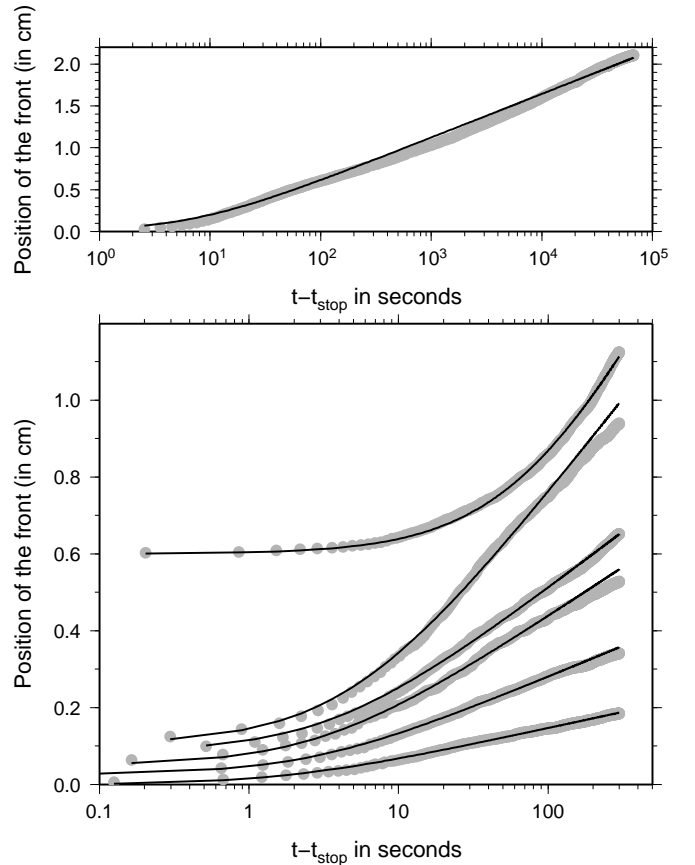
FIG. 4: Evolution of the average front position \bar{a}(t) - \bar{a}_0 during several relaxation experiments as a function of time t - t_{stop} . The observed front position is represented by gray dots while the best fits using (1) are displayed as continuous dark lines. Traces have been shifted vertically in order to enhance visibility. The experiment displayed on the top figure lasted more than 18 hours (the time representation scale is different from the one in the bottom figure).
