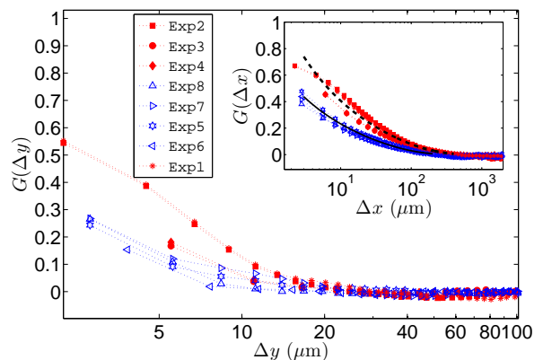
FIG. 7. (a) Time correlation functions collapsed onto each other according to a power law with an exponential cutoff G(\Delta t) = A\Delta t^{-\tau_t} \exp(-\Delta t/t^*) . The exponent is \tau_t \approx 0.43 . Inset shows the scaling between the crossover correlation time and average propagation velocity t^* \approx 7.1 \mu\text{m}/\langle v \rangle . (b) Space correlation function G(\Delta y) with logarithmic \Delta y -axis. Consistently with (a) and Eq. (7), the local velocities become uncorrelated after only a short distance ( \sim 10 - 20 \mu\text{m} ) in the y -direction. Correlation functions from experiments performed on sample #2 and #1 have filled and open markers respectively. To some extent we see also here grouping of experiments from the same sample. The difference is however not as clear as for the spatial correlations along the transverse x -axis (subparallel to the fronts), on the inset showing G(\Delta x) with logarithmic x -axis. The reason might be that the drop to zero correlation occurs close to the resolution scale for G(\Delta y) .
