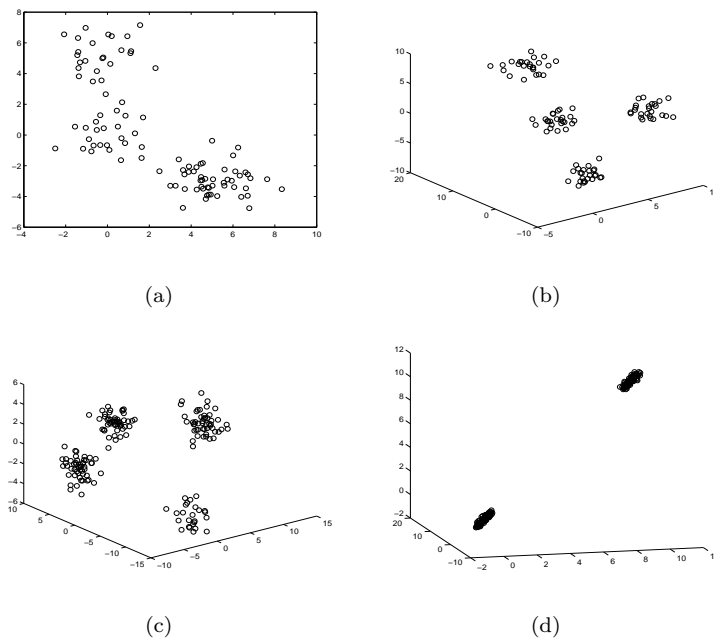
Figure 5: (a) Model 1: N = 150 ; (b) Model 2: N = 175 ; (c) Model 3: N = 175 ; (d) Model 4: N = 202
