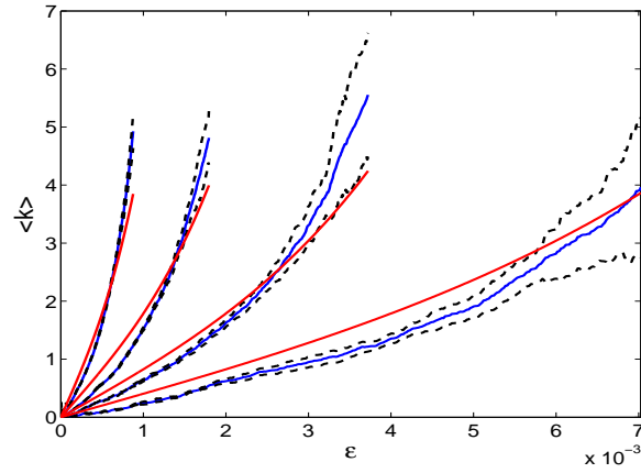
Figure 4: Average size of false alarm detected cluster from sets of uniformly distributed vertices over [0, 1]^2 , and N = 128, 256, 512, 1024 vertices respectively (curves from the right to the left). Theoretical curve (red) and numerical simulation (blue).
