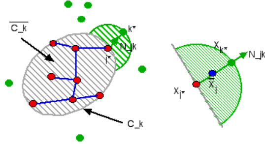
Figure 2: Left: C_k denotes the contour of the support where connected vertices are found. The neighborhood which is considered for finding a vertex that could be connected to v_i is shown. In the limit of large N , this latter neighborhood is approximated as the half sphere laying on the tangent (hyper)plane to C_k (right).
