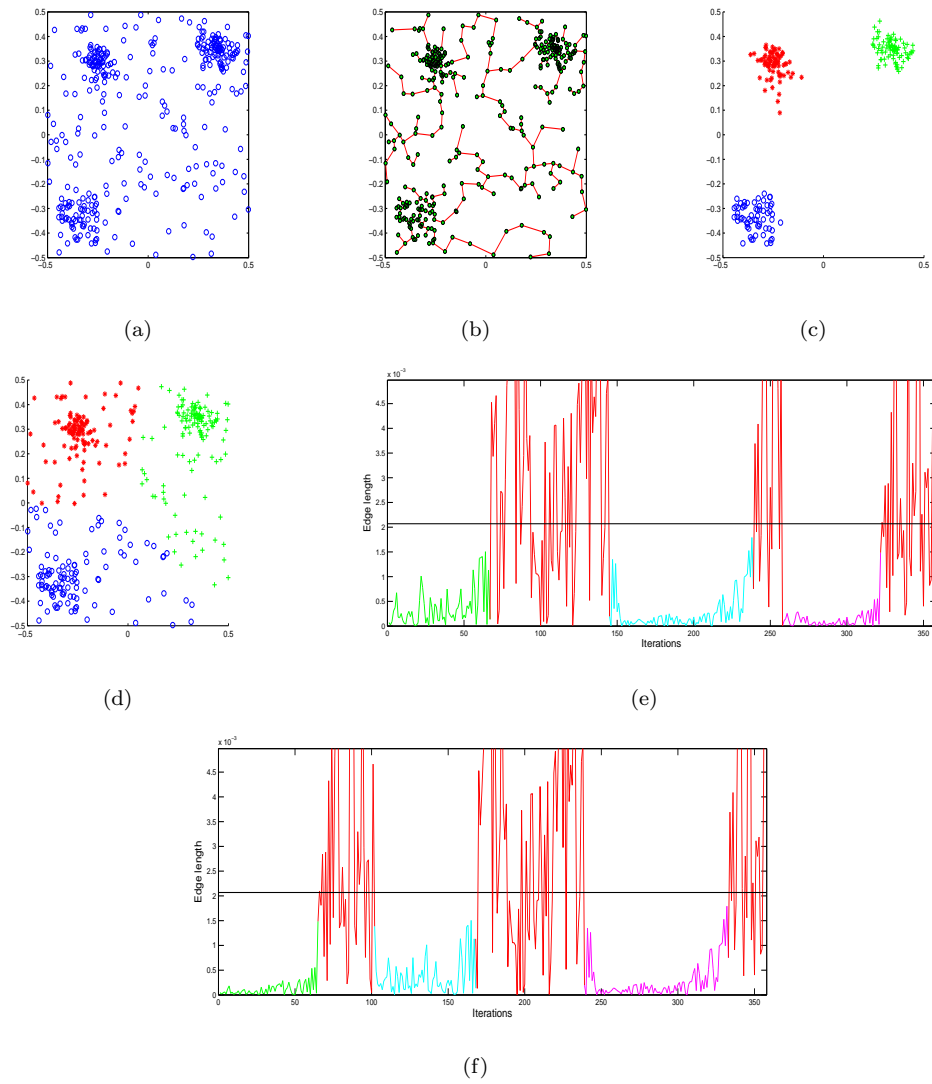
Figure 1: (a) Toy data set, (b) construction of a MST, (c) extraction of the relevant groups of vertices present below the threshold in the Prim's trajectory, (d) clustering with k-means, (e,f) Prim's trajectories with different initial vertex used in the MST construction.
