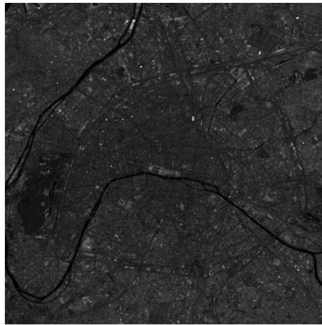
Figure 6: Multi-spectral image of Paris
