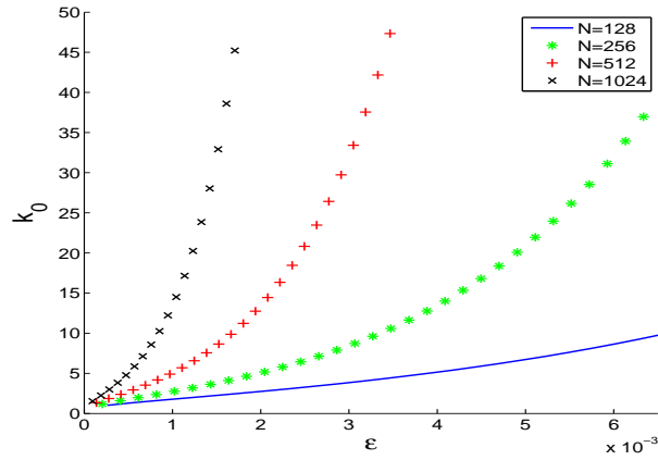
Figure 3: Minimum number of points in a detected cluster as a function of the threshold value \epsilon from sets of uniformly distributed vertices over [0, 1]^2 , for a P_{FA} = 0.05 and N = 128, 256, 512, 1024 vertices respectively.
