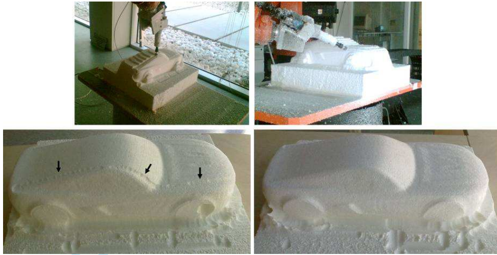
Figure 10. Milling of a small workpiece: bottom left, result without calibration; bottom right, result with calibration.
