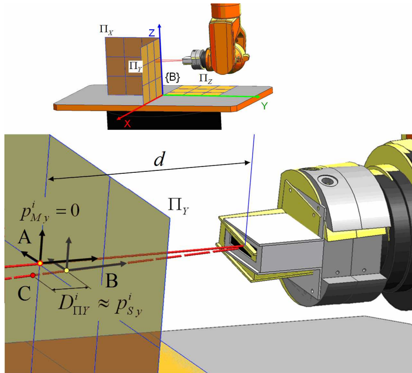
Figure 5. Three commanded meshes on the three respective planes are shown at the top; the coordinate p_S^i approximated by the distance D_{\Pi_Y}^i to \Pi_Y is shown underneath.
