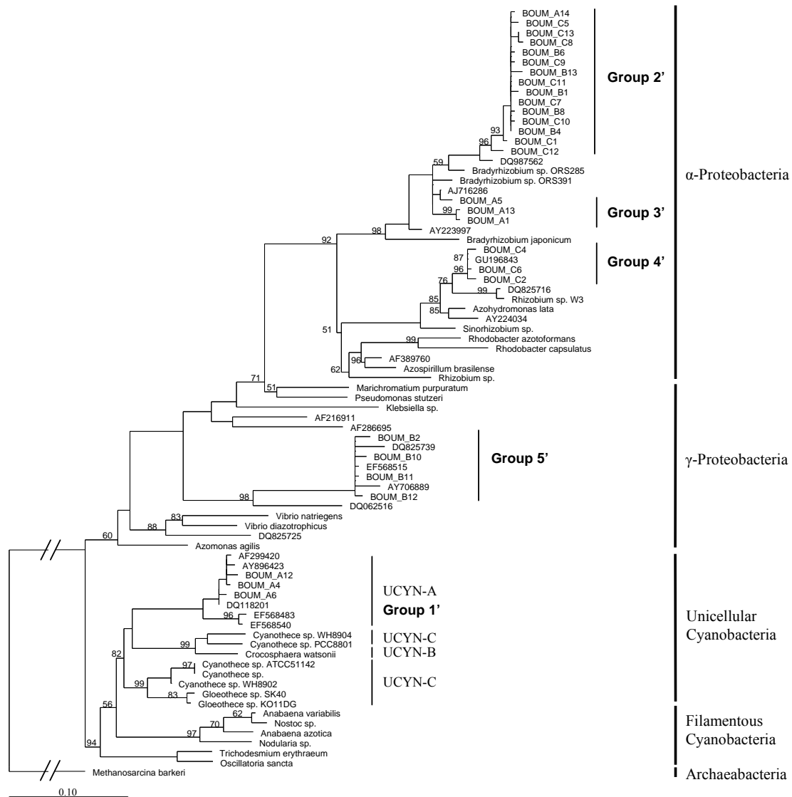
Fig. 6. Phylogenetic tree of nifH sequences. Sequences obtained in this study are referred to (i) by the oceanographic transect BOUM, (ii) the station at which they were sampled (A, B, or C), and (iii) their clone number. Bootstrap values >50% are indicated at the nodes. Scale bar = 0.1 substitution per nucleotides.
