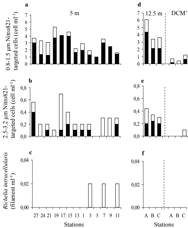
Fig. 3. Epifluorescent microscopic counts of Nitro821-targeted UCYN and filamentous diazotrophic cyanobacteria across the Mediterranean Sea within the 0.2–3 µm (black bars) and the 3–10 µm combined with >10 µm (white bars) size fractions. Counts were done at 5 m depth ( a , b , c ) and at two nutrient contrasted depths ( d , e , f ) including 12.5 m (left of dotted line) and upper deep chlorophyll maximum (DCM + , right of dotted line). Counts were done on small Nitro821-targeted cells ( a , d ), on large Nitro821-targeted cells ( b , e ), and on Richelia intracellularis ( c , f ).
