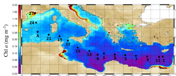
Fig. 1. Position of sampled stations during the BOUM transect across the Mediterranean Sea. Numbers (1–27) represent stations where surface TSA-FISH analyses were done and letters (A, B, and C) represent stations where TSA-FISH analyses were done at 12.5 m and DCM + as well as 16S and nifH phylogenies at 12.5 m.
