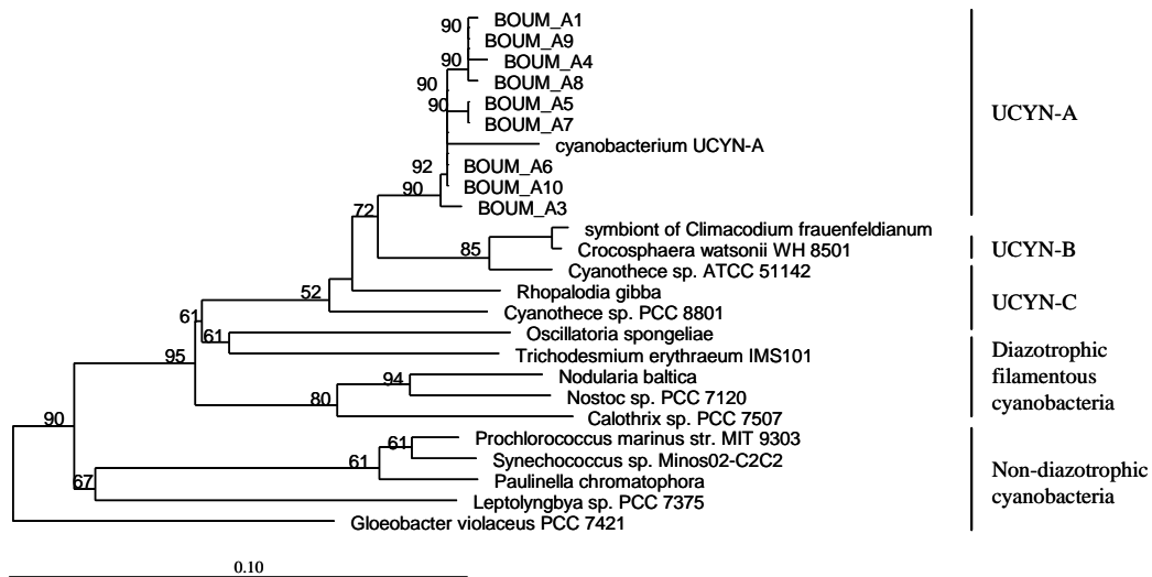
Fig. 5. Phylogenetic tree of 16S rDNA sequences from Cyanobacteria. Sequences obtained in this study are referred to (i) by the oceanographic transect BOUM, (ii) the station at which they were sampled (A, B, or C), and (iii) their clone number. Bootstrap values >50% are indicated at the nodes. Scale bar = 0.1 substitution per nucleotides.
