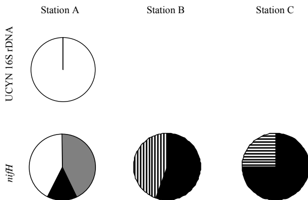
Fig. 7. Percentage of sequences from UCYN specific 16S rDNA and nifH clone libraries from station A, B, and C. Colors indicate phylogenetic groups from Figs. 5 and 6 in which sequences were recovered: UCYN-A group 1' (white); Bradyrhizobium group 2' (black); Bradyrhizobium group 3' (grey); rhizobia group 4' (horizontal lines); \gamma -proteobacteria group 5' (vertical lines).
