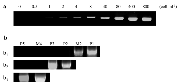
Fig. 2. Different PCR amplification tests for the detection of scarce microorganisms. (a) Definition of PCR detection limit of UCYN using a range of concentrations of C. watsonii with Nitro821/Cya359 16S primers. (b) Test of stability of PCR efficiency with time on different types of DNA template collected in the Pacific Ocean (P) or in the Mediterranean Sea (M) and stored at -80 °C for 1 to 5 yr. Amplifications were done with the general 16S primers 27F/1518R using as DNA template (b 1 ) PFA fixed cells collected on filter, (b 2 ) PFA fixed cells collected on filter and washed with MilliQ sterile water before amplification, and (b 3 ) extracted DNA.
