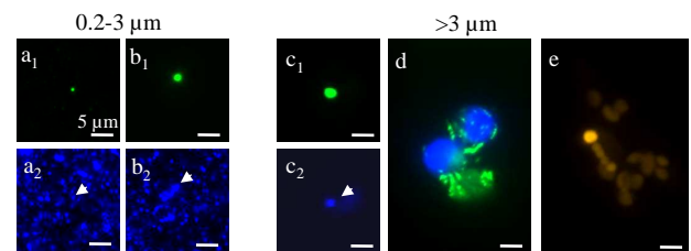
Fig. 4. Epifluorescent photomicrographs from Nitro821-targeted UCYN and filamentous diazotrophic cyanobacteria detected in the Mediterranean Sea. Nitro821-targeted UCYN were labelled with FITC (green fluorescence, a 1 , b 1 , c 1 , d ) using TSA-FISH technique. ( a 2 ), ( b 2 ), ( c 2 ) and ( d ) showed corresponding microphotograph of DAPI-stained DNA (blue fluorescence) from all prokaryotic and eukaryotic cells. Arrow heads point to the DNA from the Nitro821-targeted ones. The heterocystous Richelia intracellularis was detected owing to its natural orange fluorescence ( e ). Scale bar = 5 µm.
