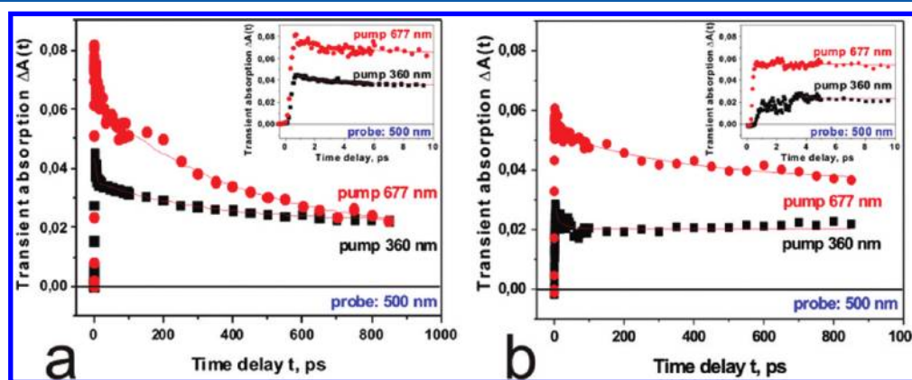
Figure 8. Transient absorption signal \Delta A(t) of AlPcS 4 in water (a) and DMSO (b) as a function time delay in the full time window up to 1 ns, probed at 500 nm, pumped at 677 and 360 nm; concentration = 10^{-3} M. The insets show the signal \Delta A(t) in the time window up to 10 ps.
