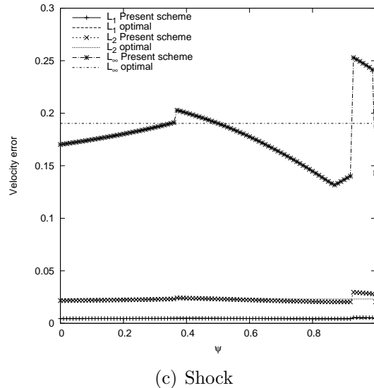
Figure 5: Present scheme error and optimal error.
