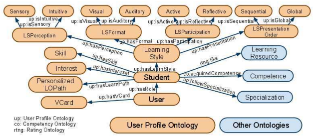
Figure 3. Part of User Profile Ontology
