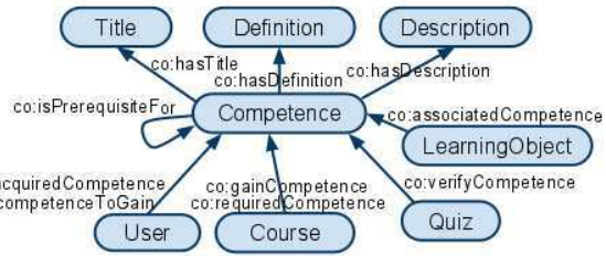
Figure 4. Part of Competency Ontology.
