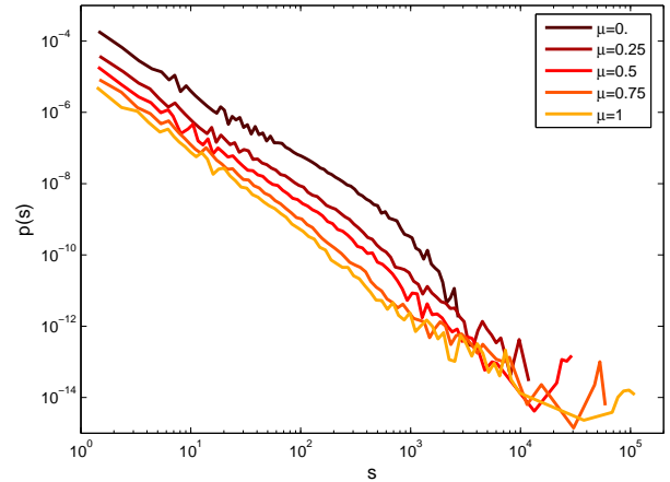
Fig. 6. Event size distribution obtained by numerical simulations for internal friction values \mu varying from 0 to 1).
