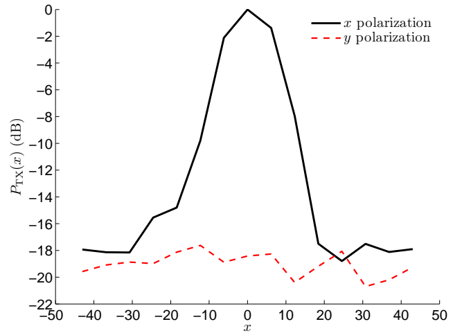
Fig. 3: Peak intensity of the signals transmitted at the interior of the EUT as a function of the focal-spot center, for two orientations of the electric field impinging over the device. The results are normalized to the value measured for a focal-spot at x = 0 , for an electric field oriented along x .
