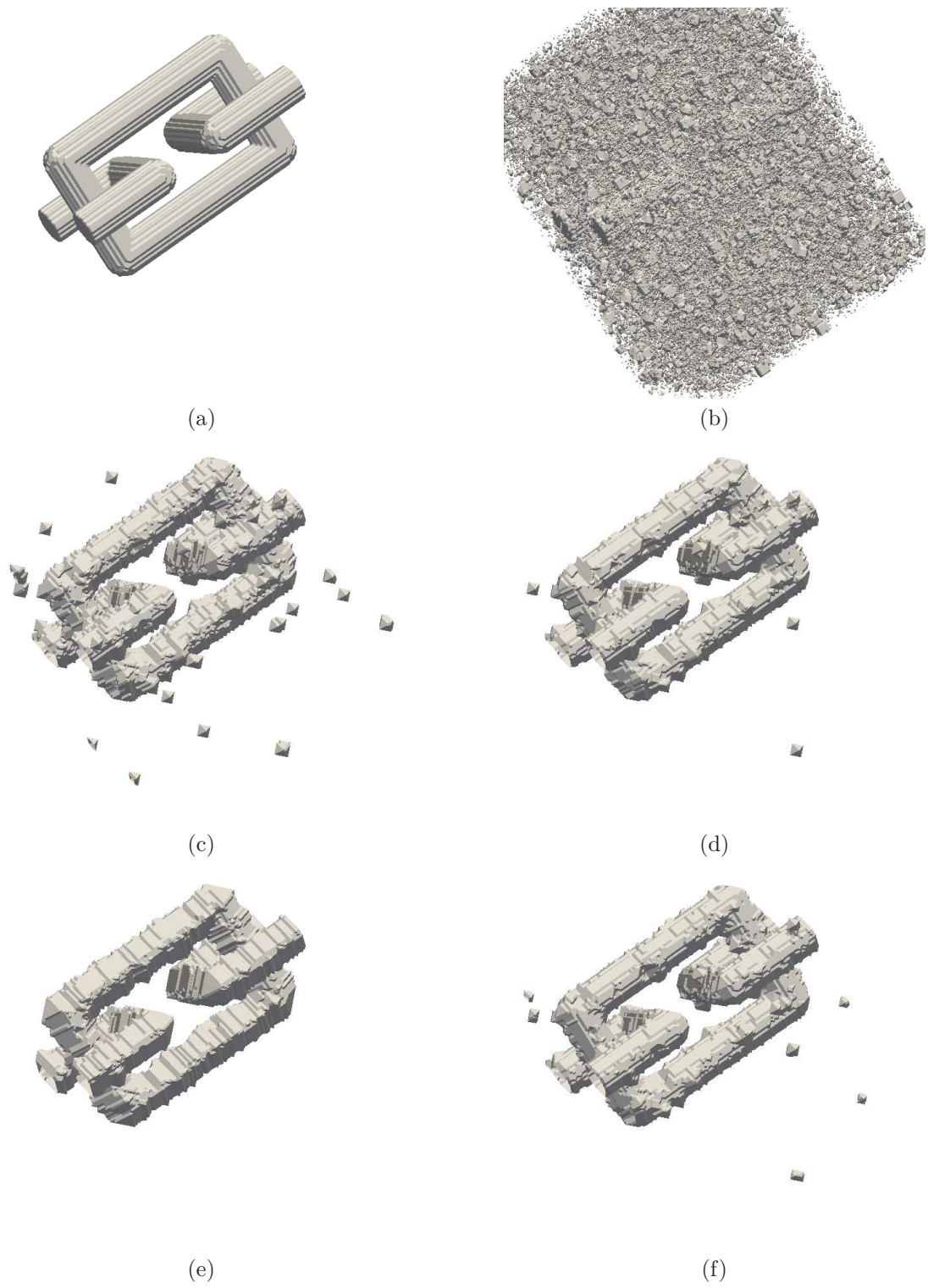
Figure 5: Same as Fig. 4 but in 3D. Rendering of: (a) original binary image, (b) noisy binary image, (c) result of usual ASF, (d) result of graph ASF, (e) result of usual ASF of double size and (f) result of usual ASF (double resolution) [see text].
