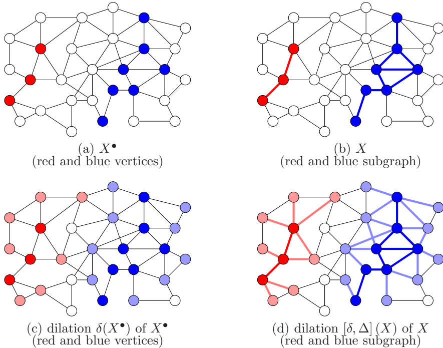
Figure 1: Illustration of a vertex-dilation and of a graph-dilation.
