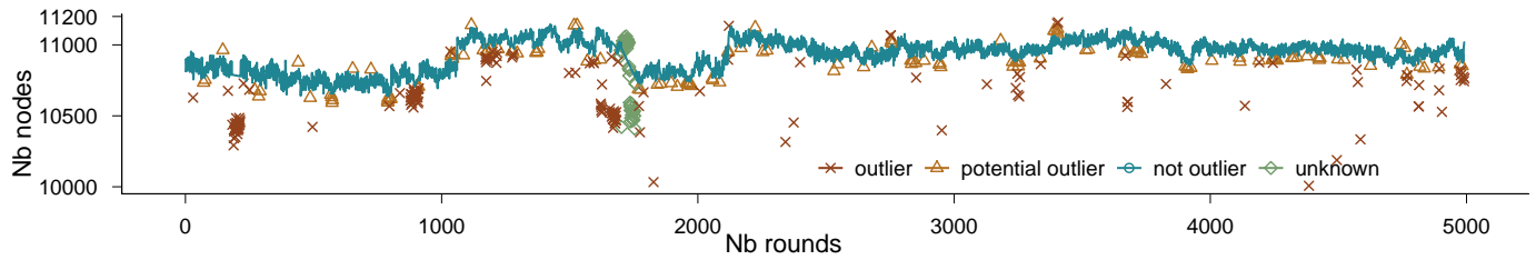
Fig. 11. Number of nodes at each round of radar measurement; outliers are detected using a sliding window of 100 rounds (25 hours).
