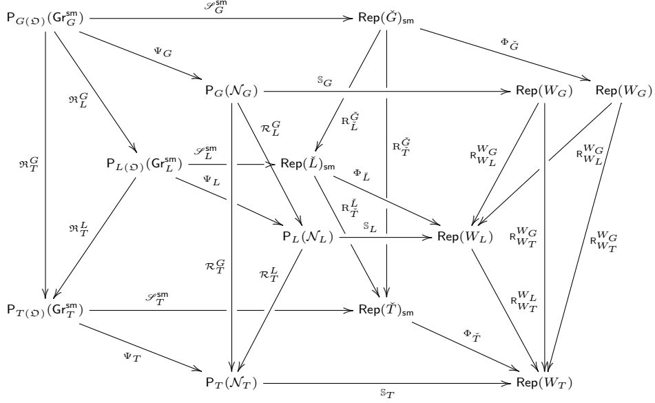
FIGURE 3.1. Diagram for the proof of Theorem 3.3. (Here, to save space, we abbreviate \mathbf{P} = \mathrm{Perv}. )
