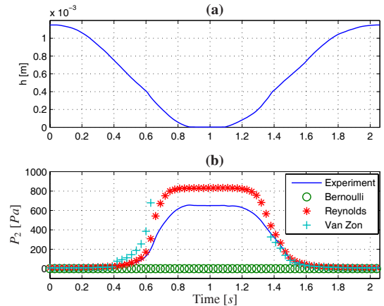
Figure 4: Experimental and theoretical results for unsteady flow, during vocal folds replica oscillation. (a) : aperture h_l of the mechanical lips. (b) : Experimental pressure P_2 and theoretical pressure P_2 computed from experimental pressure P_1 using three theoretical models : Bernoulli inviscid equation (Bernoulli), Bernoulli equation corrected for friction (Reynold), boundary layer equations (Van Zon)
