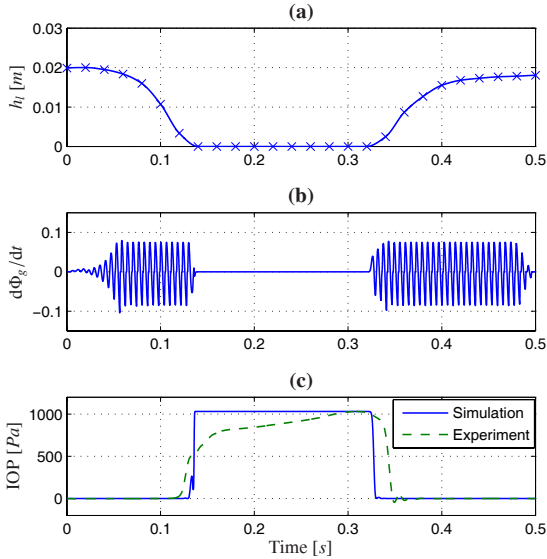
Figure 5: Numerical simulation of an /apa/ utterance. (a): h_l polynomial interpolation of lips aperture measured in vivo, represented by the crosses. (b): d\Phi_g/dt time derivative of glottis volume velocity \Phi_g simulated. (c): Comparison between simulated IOP and IOP measured in vivo.
