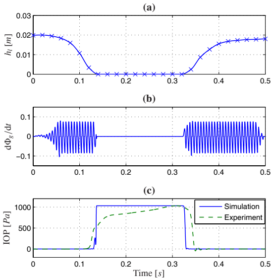
Figure 5: Numerical simulation of an /apa/ utterance. (a): h_l polynomial interpolation of lips aperture measured in vivo, represented by the crosses. (b): d\Phi_g/dt time derivative of glottis volume velocity \Phi_g simulated. (c): Comparison between simulated IOP and IOP measured in vivo.
