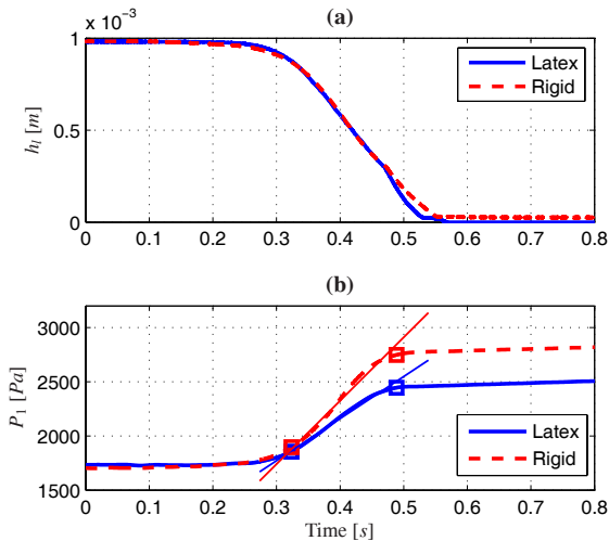
Figure 7: Influence of the expansion of latex tube during in vitro vowel-plosive-vowel utterances for the rigid tube and the deformable tube made of latex, (a): lips aperture h_l , (b): evolution of pressure P_1
