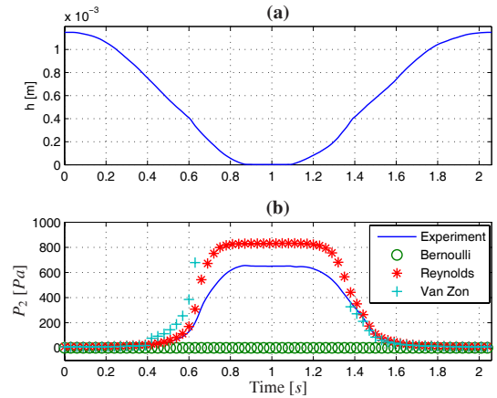
Figure 4: Experimental and theoretical results for unsteady flow, during vocal folds replica oscillation. (a) : aperture h_l of the mechanical lips. (b) : Experimental pressure P_2 and theoretical pressure P_2 computed from experimental pressure P_1 using three theoretical models : Bernoulli inviscid equation (Bernoulli), Bernoulli equation corrected for friction (Reynold), boundary layer equations (Van Zon)
