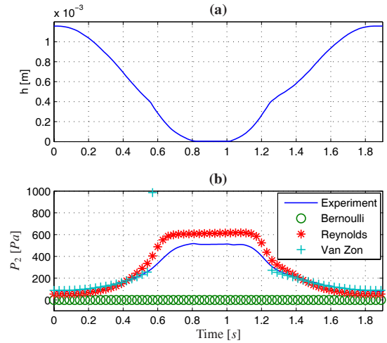
Figure 3: Experimental and theoretical results for steady flow. (a) : aperture h_l of the mechanical lips. (b) : Experimental pressure P_2 and theoretical pressure P_2 computed from experimental pressure P_1 using three theoretical models : Bernoulli inviscid equation (Bernoulli), Bernoulli equation corrected for friction (Reynold), boundary layer equations (Van Zon)
