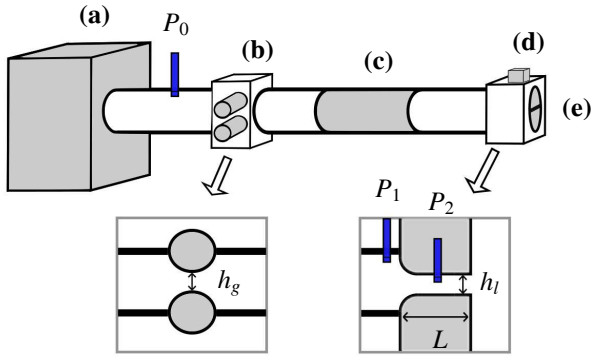
Figure 2: Replica of human phonatory system. (a) : pressure tank. (b) : replica of vocal folds. (c): plexiglas tube. (d): motor and mechanical lips displacement sensor. (e) : metal replica of lips.
