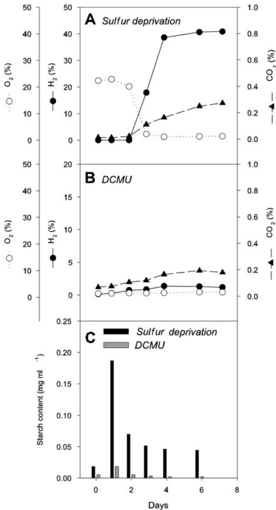
FIG. 1. Effects of DCMU on H 2 production, O 2 , CO 2 exchange, and starch accumulation in sulfur-deprived Chlamydomonas cells. (A) Control in the absence of DCMU. (B) DCMU (20 μM final concentration) was added at t 0 . Sulfur deprivation was realized by resuspending cells in sulfur-deprived TAP medium at t 0 . Relative quantities of gases contained in closed flasks were measured by mass spectrometry and are expressed as the percentage of the gas phase volume. (C) Intracellular starch amounts measured at different times in the culture conditions described for panels A and B.
