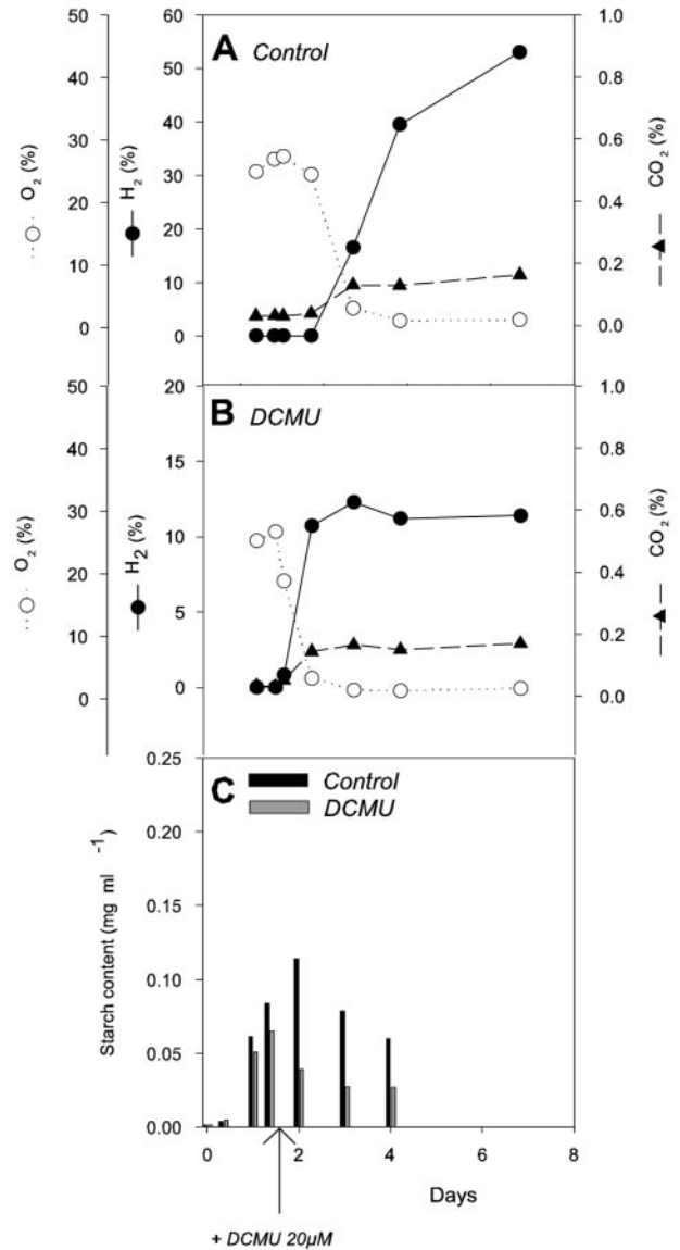
FIG. 2. Effects of retarded DCMU addition on H 2 production, O 2 , CO 2 exchange, and starch accumulation in sulfur-deprived Chlamydomonas cells. (A) Control in the absence of DCMU. (B) DCMU (20 μM final concentration) was added 24 h after the beginning of sulfur deprivation. (C) Intracellular starch amounts measured at different times in the culture conditions described for panels A and B. Other experimental conditions are similar to those described for Fig. 1.
