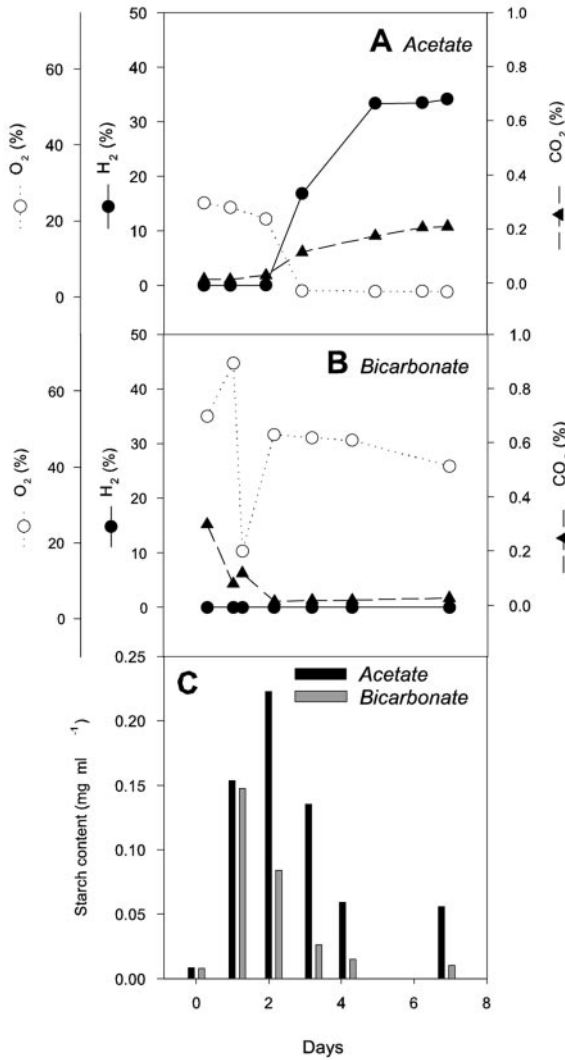
FIG. 3. Effects of acetate on H_2 production, O_2 , CO_2 exchange, and starch accumulation in sulfur-deprived Chlamydomonas cells. (A) Control in the presence of acetate (TAP medium). (B) Acetate was omitted from the culture medium (minimal medium supplemented with 20 mM bicarbonate); in this experiment, N_2 bubbling was achieved 24 h after the beginning of sulfur deprivation. For both experiments, sulfur deprivation was achieved at t_0 . (C) Intracellular starch amounts measured at different times in the culture conditions described for panels A and B.
