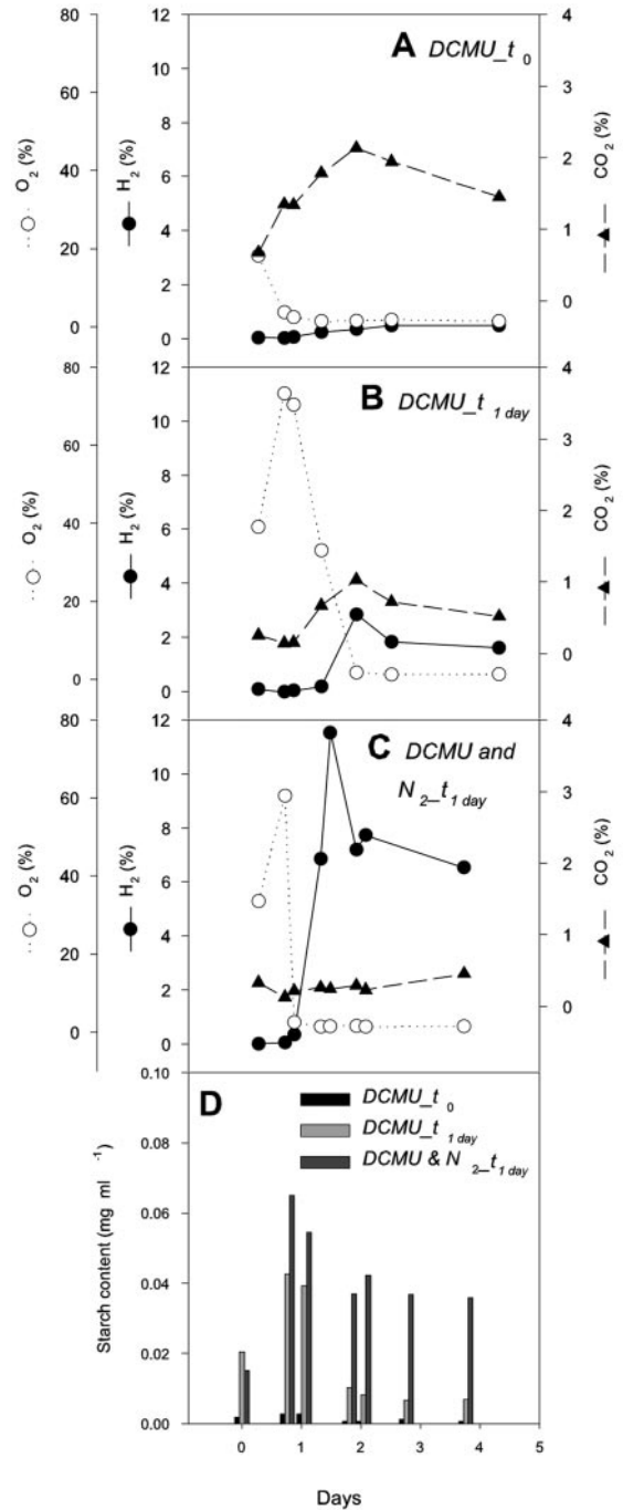
FIG. 4. Effects of DCMU addition and N_2 flushing on H_2 production, O_2 , CO_2 exchange, and starch accumulation by Chlamydomonas cells in sulfur-deprived minimal medium supplemented with 20 mM bicarbonate. (A) DCMU was added at t_0 , (B) DCMU was added at 24 h, and (C) DCMU was injected and N_2 bubbling was performed at 24 h. For the three experiments, sulfur deprivation was achieved at t_0 . (D) Intracellular starch amounts measured at different times in the culture conditions described for panels A, B, and C.
