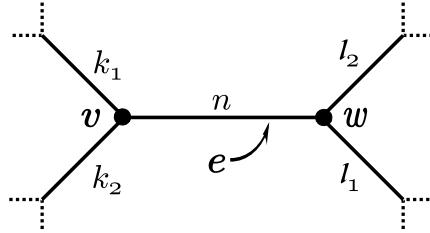
Figure 2: A ridge of type \langle k_1, k_2, n, l_1, l_2 \rangle
