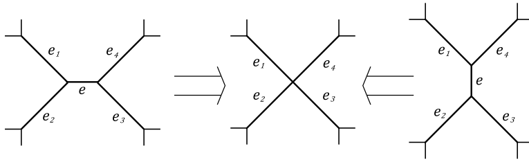
Figure 6: Two possible ridges resulting in a four-valent vertex under contraction
