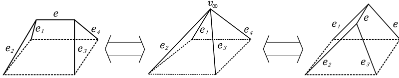
Figure 7: Pushing together and pulling apart the supporting planes of polyhedron's faces results in an “edge contraction”- “edge insertion” process
