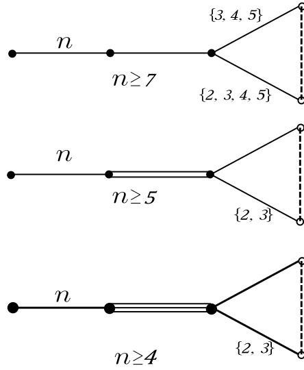
Figure 14: Prisms that admit contraction of an edge: the first picture
