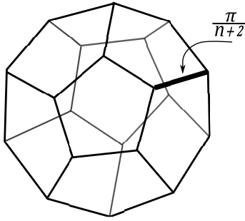
Figure 1: The dodecahedron \mathcal{D}_n \subset \mathbb{H}^3 , n \geq 0 , with all but one right dihedral angles. The specified angle equals \frac{\pi}{n+2}
