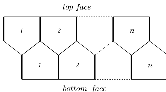
Figure 12: Löbell polyhedron L(n) , n \geq 5 with one of its perfect matchings marked with thickened edges. Left- and right-hand side edges are identified
