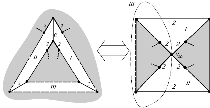
Figure 9: Forbidden 3-circuit: the second case. The forbidden circuit going through the ideal vertex is dotted. Face III is at the back of the picture
