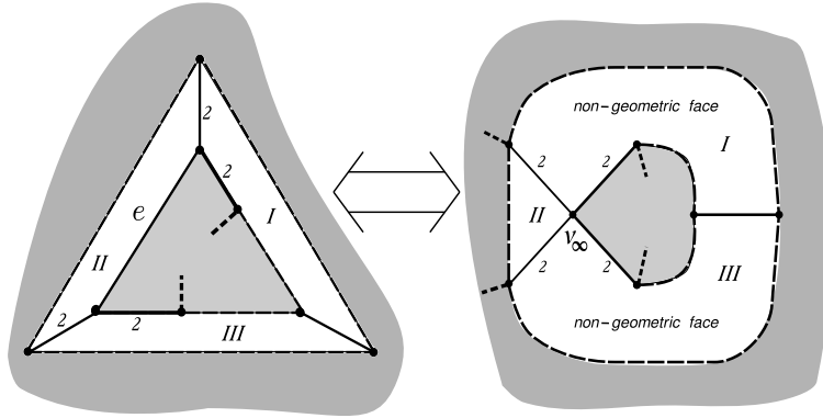
Figure 8: Forbidden 3-circuit: the first case
