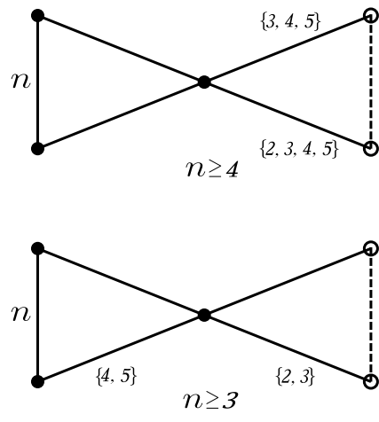
Figure 16: Prisms that admit contraction of an edge: the third picture
