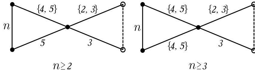
Figure 15: Prisms that admit contraction of an edge: the second picture
