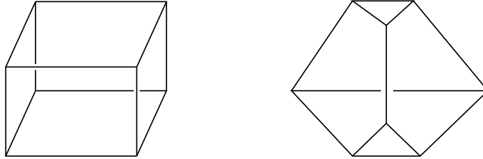
Figure 11: Simple polyhedra with eight vertices
