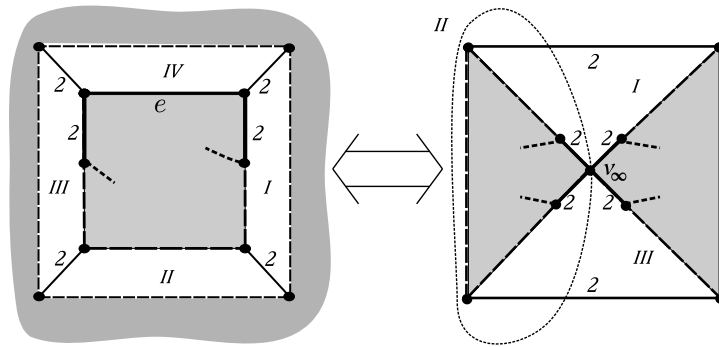
Figure 10: Forbidden 4-circuit. The forbidden circuit going through the ideal vertex is dotted. Face II is at the back of the picture
