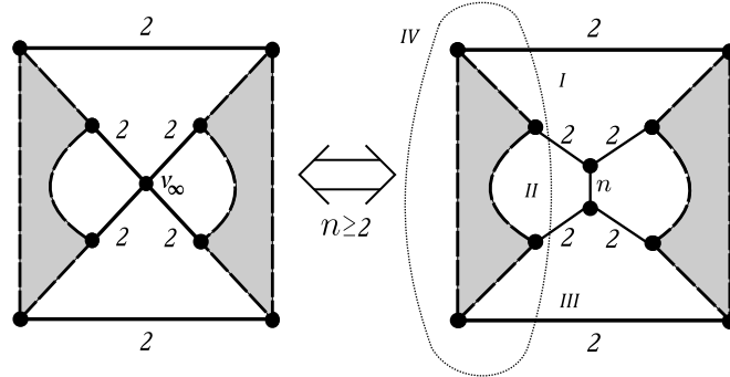
Figure 4: The first possible position of the contracted edge e . The forbidden 4-circuit is dotted. Face IV is at the back of the picture
