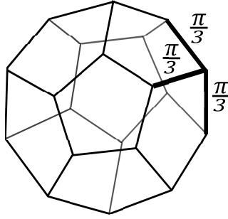
Figure 13: The dodecahedron \mathcal{D} with one ideal three-valent vertex
