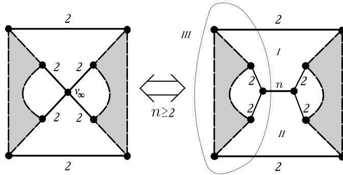
Figure 5: The second possible position of the contracted edge e . The forbidden 3-circuit is dotted. Face III is at the back of the picture
