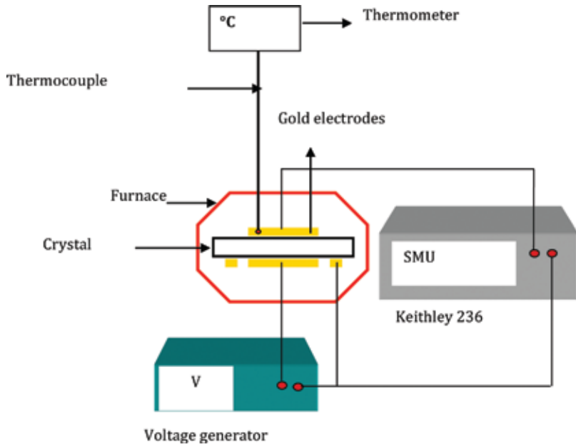
FIGURE 3 Setup measurement performed for volumic dielectric conductivity.
