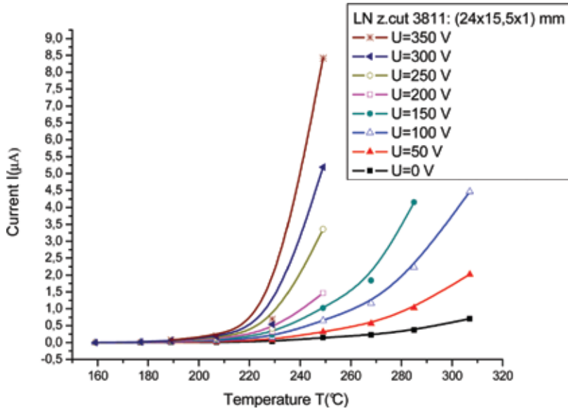
FIGURE 6 I-T characteristics of the LN sample for various applied voltage up to 350V.
