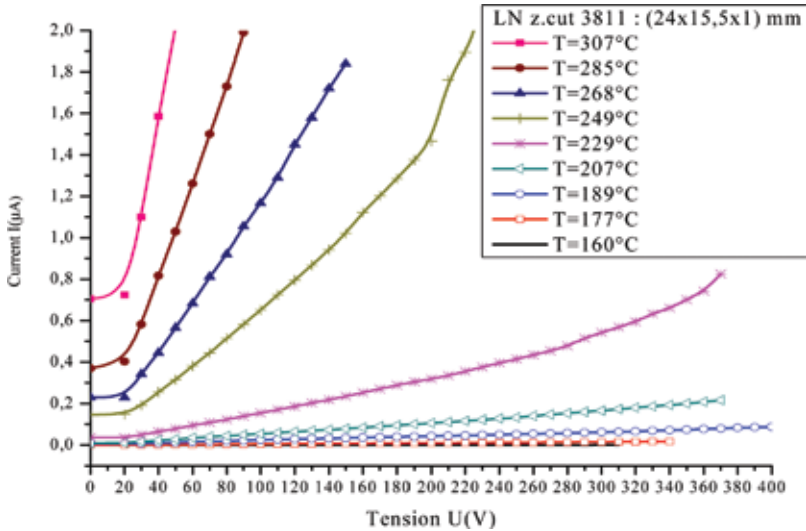
FIGURE 5 I-V characteristics of the LN sample for various temperatures up to 300°C.
