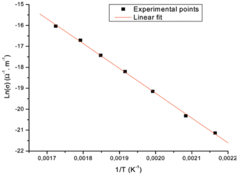
FIGURE 8 Electric conductivity of the LN sample in the 189°-300°C temperature range.
