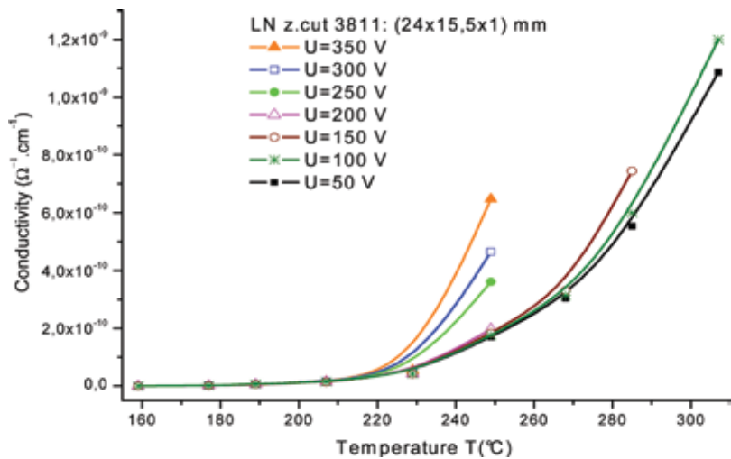
FIGURE 7 Electric conductivity of the LN sample as function of the temperature for various applied voltage.
