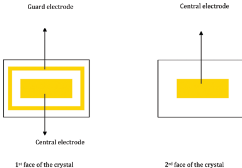
FIGURE 1 Geometrical configuration of the electrodes on the sample under test.
