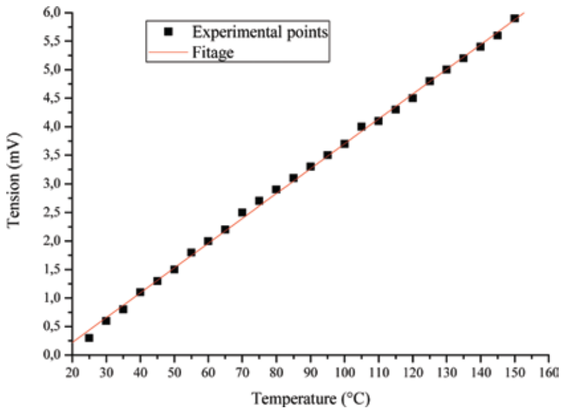
FIGURE 4 Oven calibration: V-T characteristic of the thermocouple up to 160°C.
