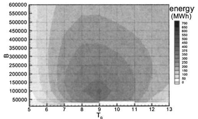
Fig. 17 Influence of B and T_0 on annual energy production (uncontrolled device), T_s=9 s, H_s=1.5 m
