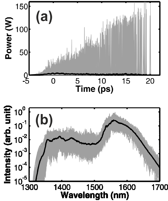
Figure 4: Superposition of 200 simulations of the output temporal (a) and spectral (b) intensity profiles of a secant hyperbolic pulse (FWHM duration of 3 ps, peak power of 10 W) propagating in a 500-m highly nonlinear fiber (nonlinear coefficient 10 /W/km, dispersion 0.5 ps/nm/km, dispersion slope 0.01 ps/nm/km at 1550 nm). Results are obtained by the numerical integration of the standard NLSE with third-order dispersion and include the quantum noise as well as 1% of the fluctuations on the input pump. The different shots are plotted in grey and the average curve is plotted with a solid black line.
