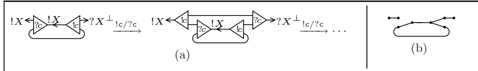
Fig. 5: a simple net not enjoying cut-elimination, nor switching acyclicity.
