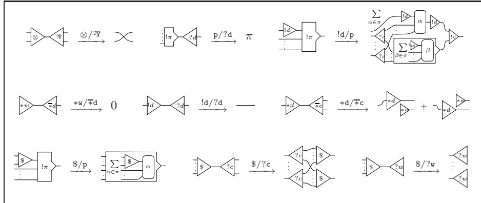
Fig. 4: elementary reduction steps (ers) for differential nets, where * (resp. \bar{*} ) is ? (resp. !) or ! (resp. ?), and \$ is !w , or !c , or !π . In the !w/?w ers the contractum is the empty graph.
