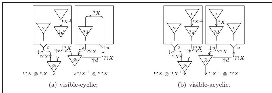
Figure 6: example of the importance of directedness in the notion of visibility.
