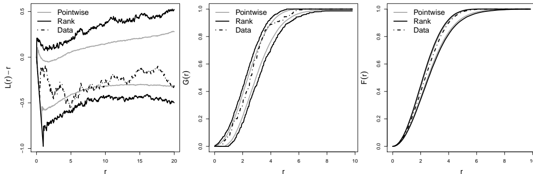
Figure 9: Left to right: Non-parametric estimate of L(r) - r , G(r) and F(r) for the oak and beech dataset with simulation based envelopes for the fitted Whittle-Matérn DPP model. The envelopes are 2.5% and 97.5% pointwise quantiles (gray lines) and rank envelopes with a 5% significance level (black lines). Both sets of envelopes are based on 4000 simulated realizations.
