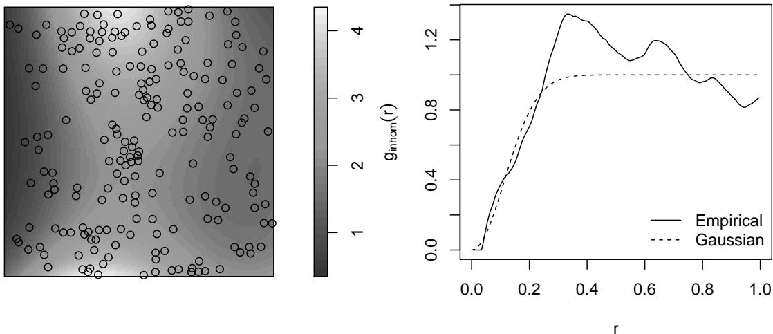
Figure 11: Japanese pines dataset. Left: Estimated intensity function \rho_{\hat{\psi}} with the points of the dataset overlaid. Right: Empirical pair correlation function and theoretical pair correlation function for the fitted Gaussian DPP model.
