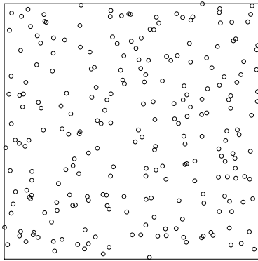
(c) Locations of 244 trees of the species oak and beech in an 80 m by 80 m region.
