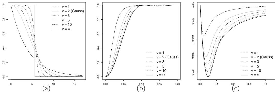
Figure 5: (a) Isotropic spectral densities, (b) approximate isotropic pair correlation functions, and (c) approximate L(r) - r functions for power exponential models with \rho = 100 , \nu = 1, 2, 3, 5, 10, \infty and \alpha = \alpha_{\max} the maximal permissible value determined by (5.34).
