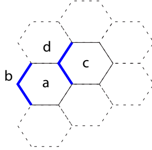
FIG. 5.3. Description of the propagation operator
