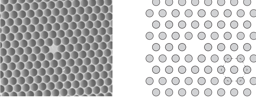
FIG. 1.1. A locally perturbed photonic crystal with triangular lattice (cross section of a photonic crystal optical fiber (left) and representation of the corresponding hexagonal periodicity cell (right)).
