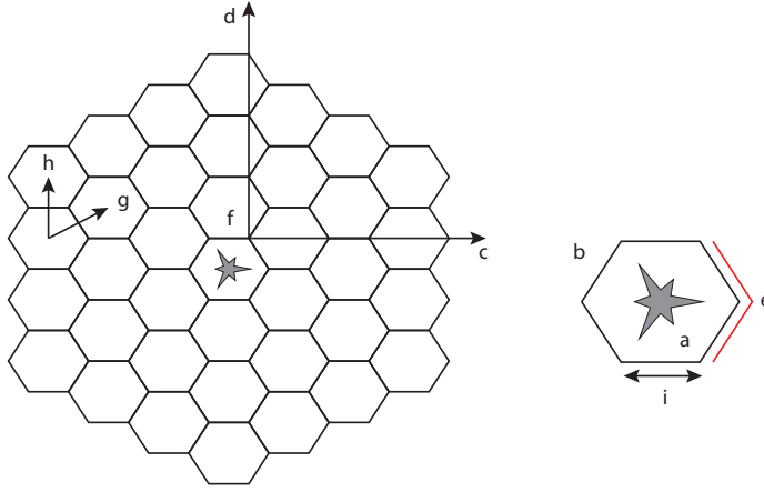
FIG. 1.2. The hexagonal periodic medium with defect.
