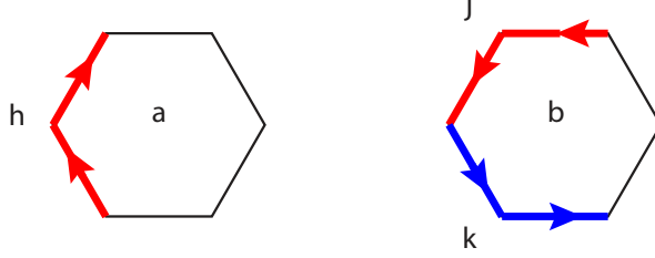
FIG. 5.2. Notations used for a periodicity cell
