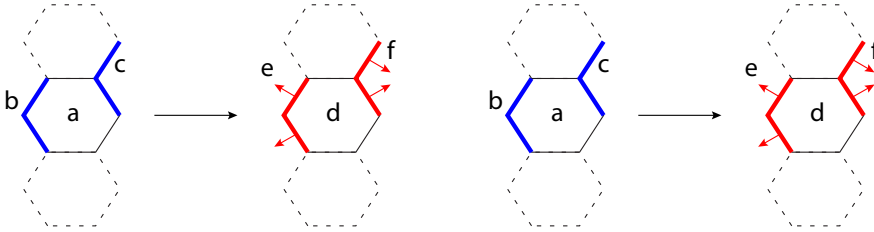
FIG. 5.5. The four local DtN operators
