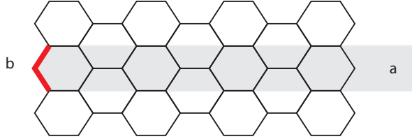
FIG. 5.1. The domain \Omega^W and its left boundary \Sigma_{00}^\ell .
