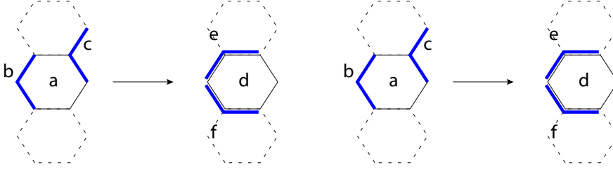
FIG. 5.6. The four local DtD operators
