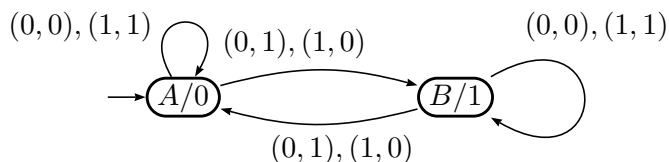
FIGURE 5. A 2-dimensional 2-automaton generating the map f defined in Example 5.7.
