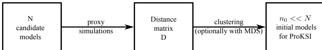
Figure 1: Initialization steps of the ProKSI algorithm.
