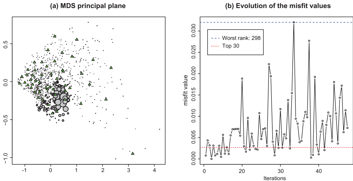
Figure 6: (a) Every point in the MDS space represents a parameter field. The triangles indicate the models that were selected by the K-means algorithm for the initial design of experiments, and the radius of the circles are proportional to the EI_\alpha criterion; (b) Monitoring of the misfit values obtained for the parameter fields sequentially chosen by the ProKSI algorithm.
