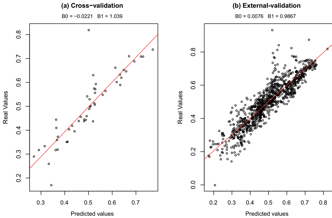
Figure 9: (a) Cross validation and (b) External validation
