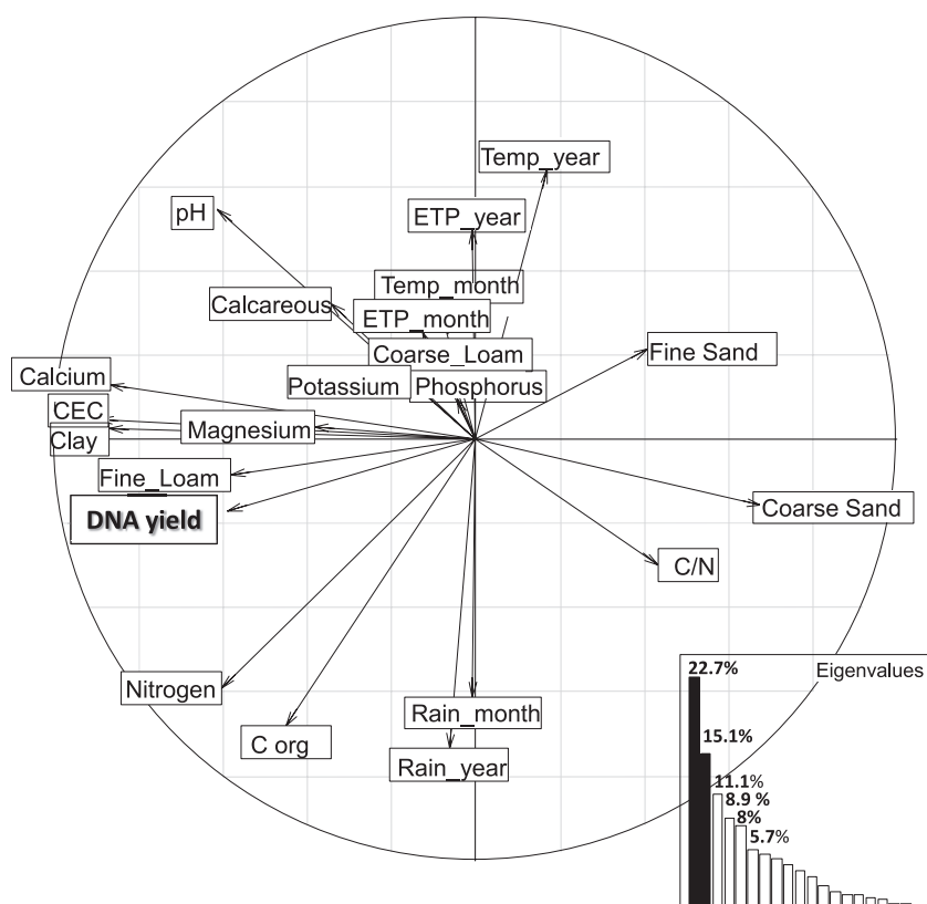
Figure 5 Correlation circle of the principal components analysis (PCA) on the correlation matrix of soil physicochemical characteristics, climatic conditions and DNA recovery data, showing factors contributing to distinction between the soil samples. C/N, carbon to nitrogen ratio; ETP, evapotranspiration; Temp, atmospheric temperature; CEC, cation exchange capacity.
