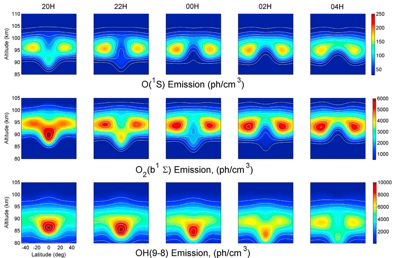
Figure 8. Model results of O(^1S) , O_2(b^1\Sigma) , and OH(9-8) emission corresponding to the WINDII observations of Figure 7 [from Ward, 1999 ]. This is for a diurnal tide of average amplitude, with latitude structure given by the (1,1) Hough mode, the accepted airglow chemistry [ McDade, 1997 ], and vertical wavelength and phase appropriate to the equinox conditions for the hydroxyl emission shown in Figure 7.
