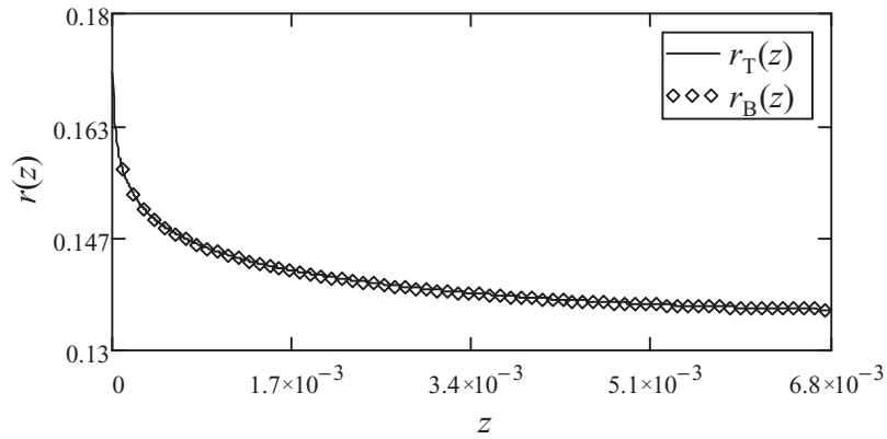
Figure 8.8 Meniscus profiles r_T (8.36) and r_B (8.38) vs z .
