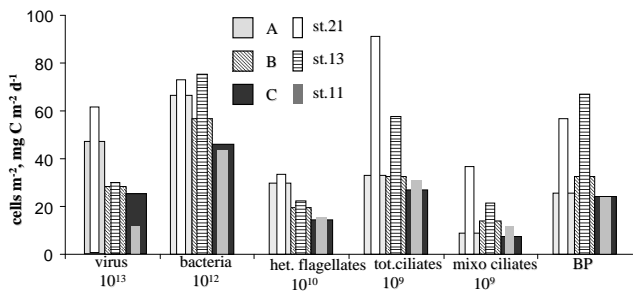
Fig. 5. Integrated values of viral particles ( 10^{13} \text{ m}^{-2} ), heterotrophic bacteria ( 10^{12} \text{ m}^{-2} ), heterotrophic nanoflagellates ( 10^{10} \text{ m}^{-2} ), total ciliates ( 10^9 \text{ m}^{-2} ) and mixotrophic ciliates ( 10^9 \text{ m}^{-2} ) and bacterial production (BP, \text{mg C m}^{-2} \text{ d}^{-1} ) in the upper 150 m, inside the eddies Sites A, B and C and outside the eddies St. 21, 13 and 11 respectively.
