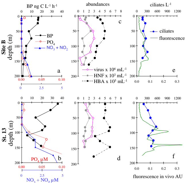
Fig. 7. Profiles of bacterial production ( \text{ng CL}^{-1} \text{ h}^{-1} ), \text{PO}_4 and \text{NO}_2 + \text{NO}_3 ( \mu\text{M} ) (a, b), viral (VLP, 10^6 \text{ mL}^{-1} ), bacterial (HBA, 10^5 \text{ mL}^{-1} ) and heterotrophic nanoflagellate abundance (HNF, 10^3 \text{ mL}^{-1} ), (c, d), ciliate abundance ( \text{L}^{-1} ) and in situ fluorescence (e, f) in the centre of the eddy B (upper panel a, c, and f) and at St. 13 (lower panel b, d and e).
