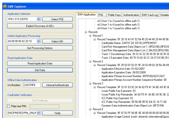
FIGURE 7. Le plugin "EMV Explorer"
