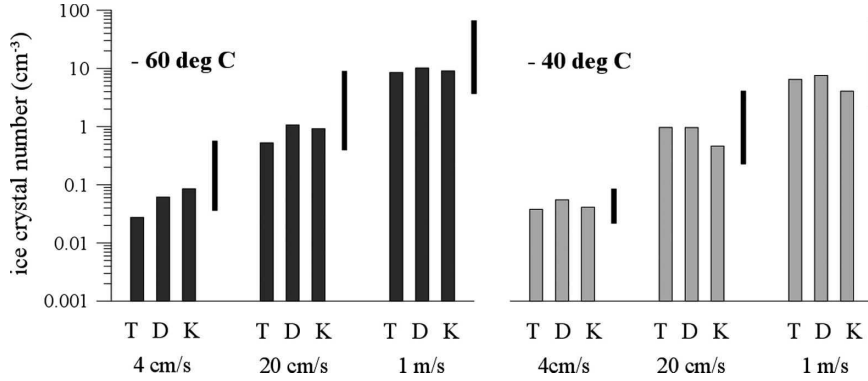
FIG. 3. Total number of ice crystals formed by homogeneous nucleation using different vertical updraft velocities, w , and different nucleation rates from TAB (T), KOO (K), or DEM (D). The black bars represent the range of results found in Lin et al. (2002) for the same scenarios.
