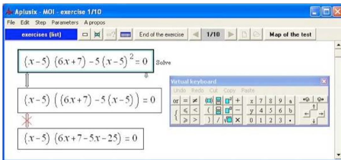
Figure 1 : Aplusix
