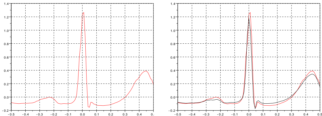
FIGURE 7. Estimation of f by \widehat{f}_n (in red) and with the mean average signal (in black)
