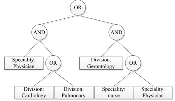
Fig. 2. An access tree T
