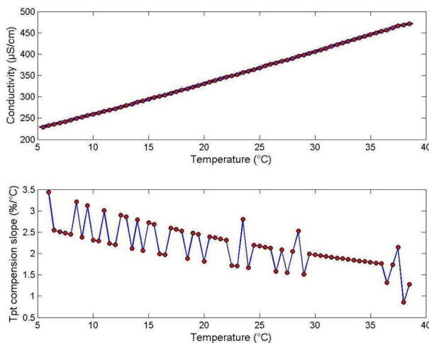
FIGURE 5 – Top : water conductivity versus temperature ; bottom : temperature compensation slope versus temperature
