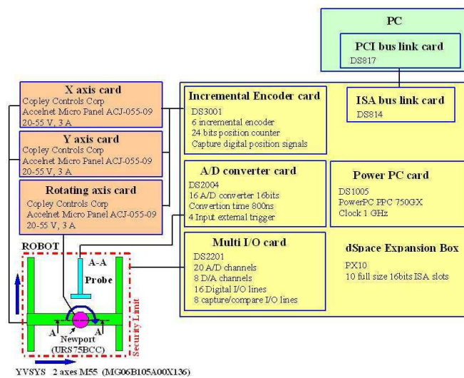
FIGURE 14 – Computer monitoring of the test bench.
