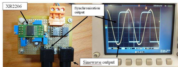
FIGURE 8 – Prototype circuit of embedded generator and test result.
