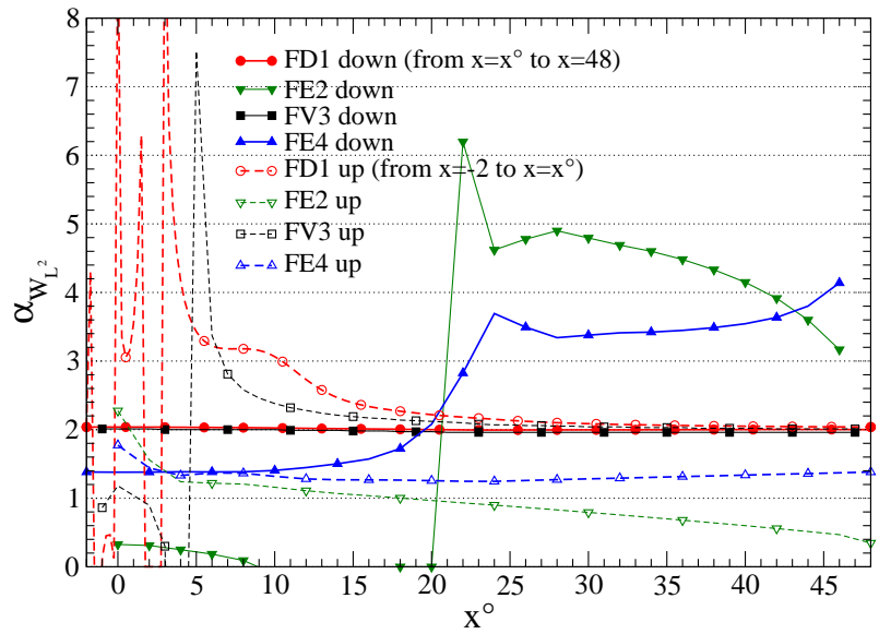
(c) L^2 norm of vertical velocity component W_{L^2}
