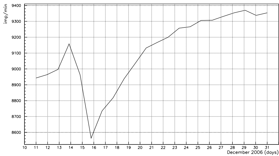
Figure 4: Moscow neutron monitor counting rate in December 2006 [32]. A Forbush decrease occurred on December 15th. We recall that the neutron monitor countrate (Y-axis label) is expressed in neutron impulses per minute.
