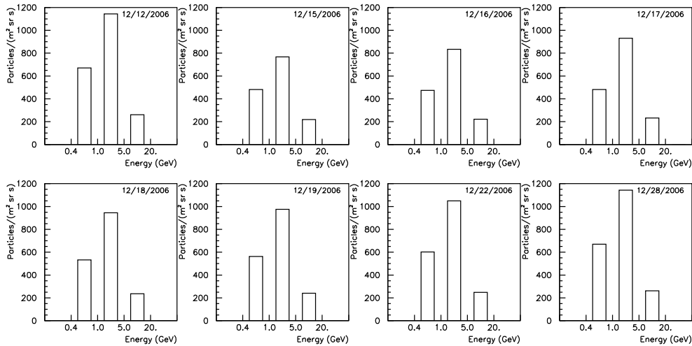
Figure 6: GCR integral proton flux observed by PAMELA in various energy intervals between December 12th and December 28th 2006 [37].
