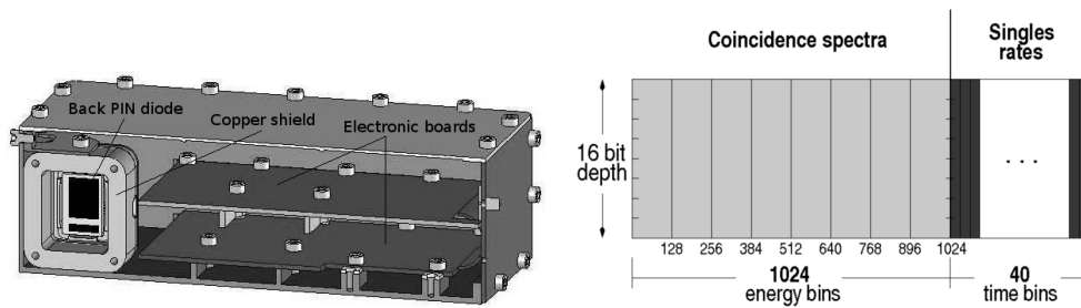
Figure 6. Left panel: schematics of the Radiation Monitor. Right panel: the Radiation Monitor data histogram, including 1024 energy bins for coincident events and 40 bins for singles counts —see text for more details.
