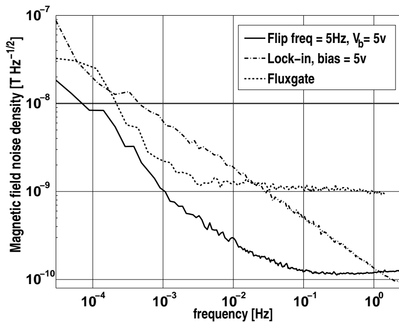
Figure 4. Magnetometers sensitivity curves. The horizontal, thicker grey line at 10^{-8} \text{Tesla Hz}^{-1/2} is the current LPF magnetometer noise requirement, which is comfortably met in all cases considered, i.e., for frequencies above 1 mHz. The curves show that the best performance corresponds to the AMR with a flip voltage scheme, showing significant improvements over the more conservative lock-in approach. The Fluxgate performs well but is slightly noisier at LISA frequencies.
