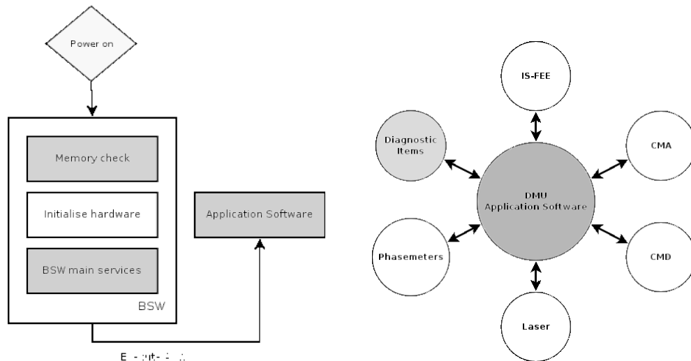
Figure 9. Conceptual diagram of the DMU software: BSW on the left and ASW on the right.
