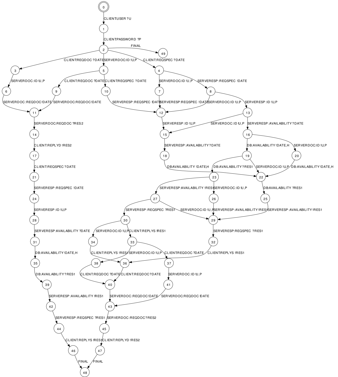
Figure 12: Adaptor protocol generated for the Online Medical System example
