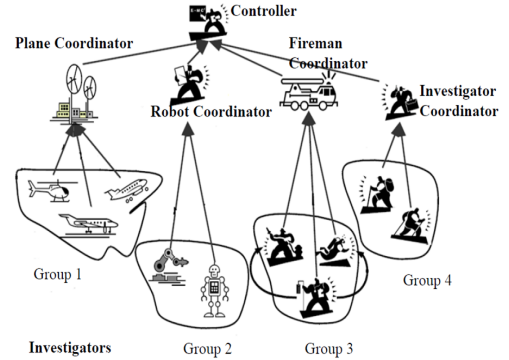
Figure 4. CMS architecture
