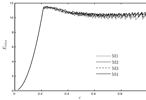
Figure 12. Change of elastic energy stored in the structure with a load increase from c = 0 to c = 1 for different meshes.
