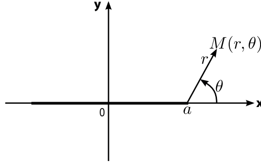
Figure 1. Definition of a basis at the crack tip.
