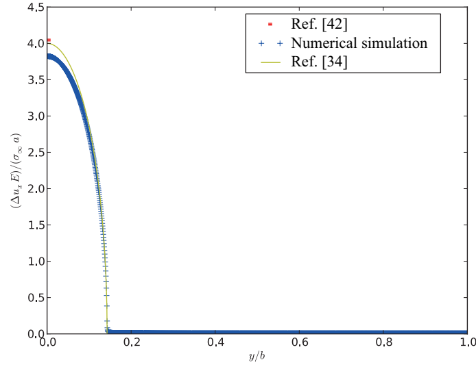
Figure 7. Comparison between the simulated and analytical crack opening displacement ( a/b = 0.14 , \ell_c = 20 mm).
