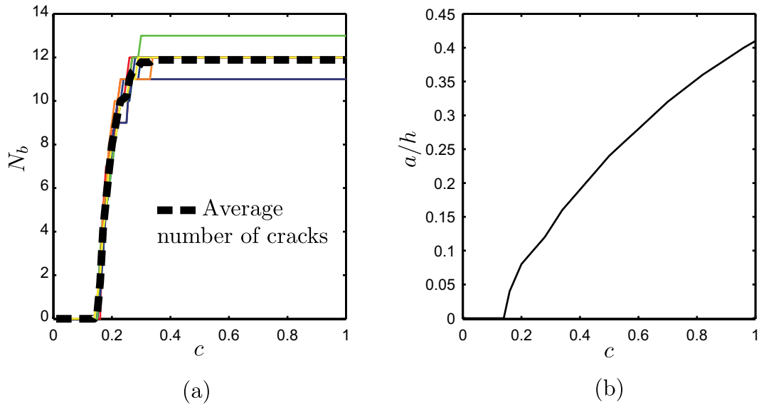
Figure 15. Change of the number of propagating cracks N_b with the applied load c for each random selection, and average value (a). Change of the average normalized length of propagating cracks a/h (b).
