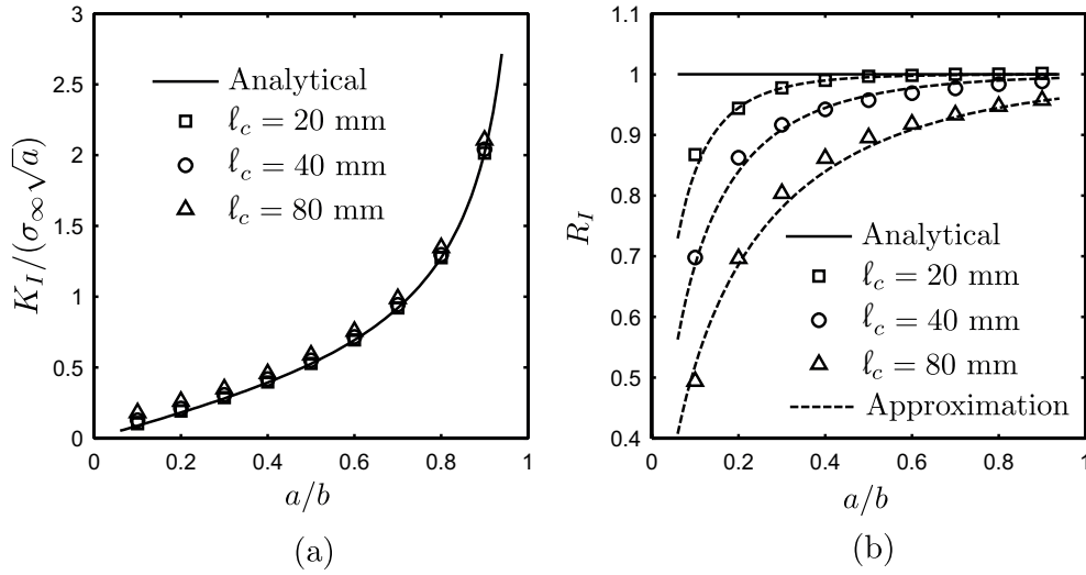
Figure 5. Stress intensity factors (a) and difference between analytical and nonlocal estimations (b) as functions of normalized crack lengths for different characteristic lengths. The proposed approximation (40) is also drawn (b).
