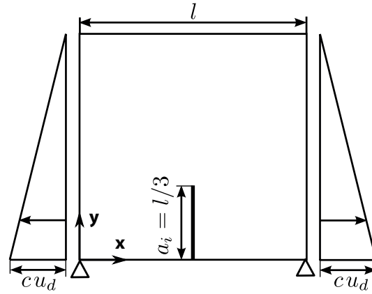
Figure 9. Schematic of the studied case.
