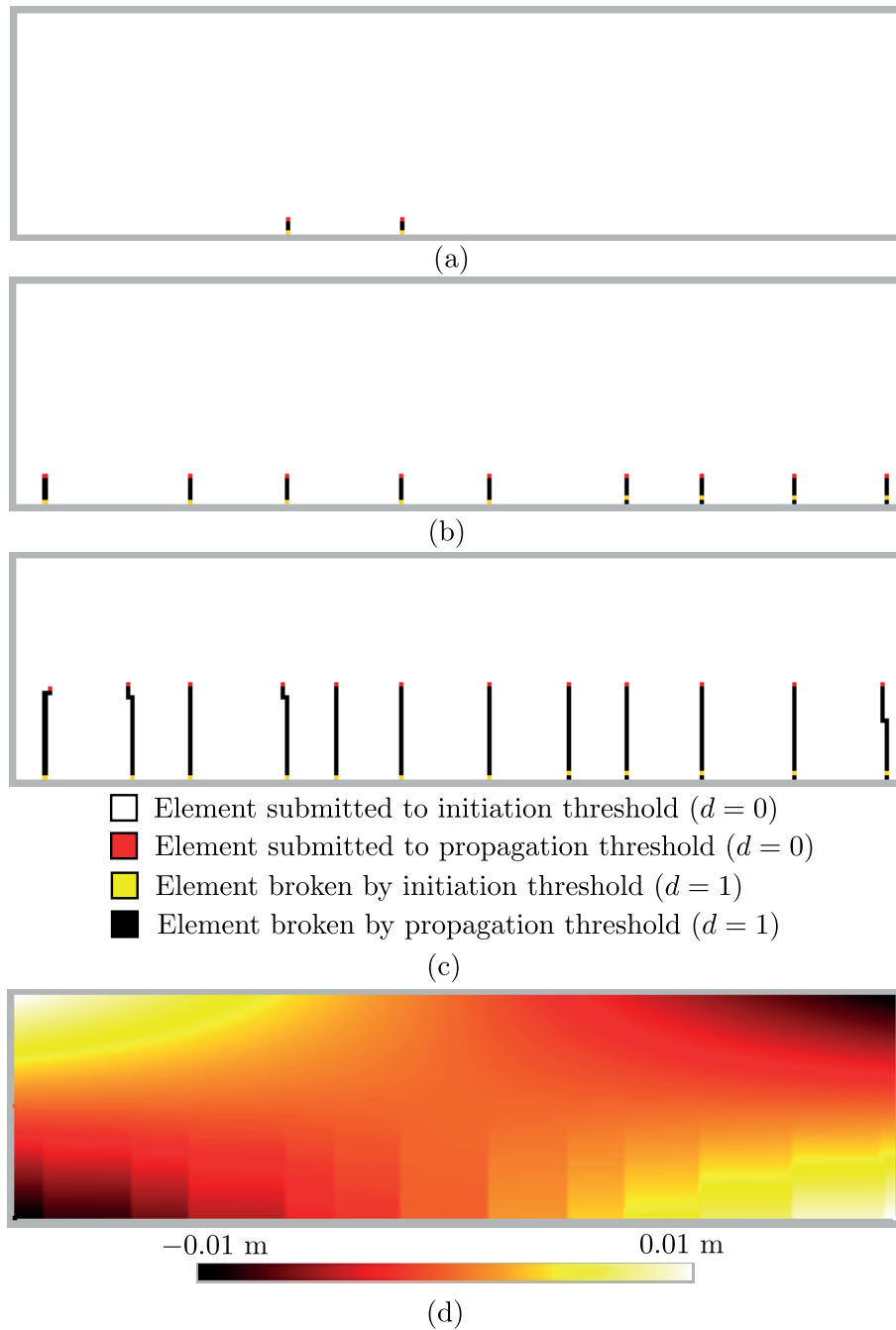
Figure 14. Finite element state for different loading levels c = 0.16 (a), c = 0.25 (b), c = 1 (c) and horizontal displacement field for c = 1 (d).
