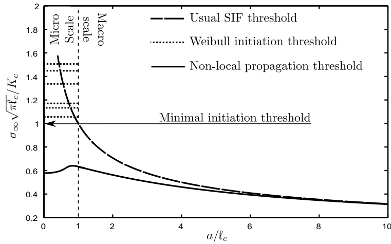
Figure 6. Change of the considered thresholds with normalized crack (or defect) size.
