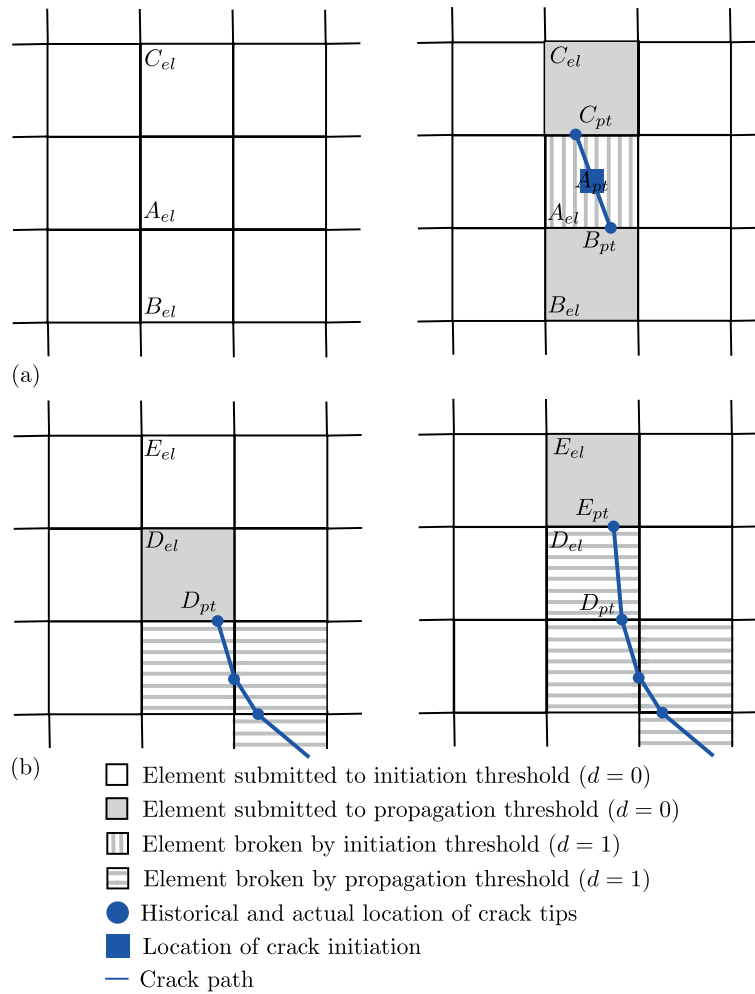
Figure 3. Numerical discretization of crack initiation (a) and growth (b).
