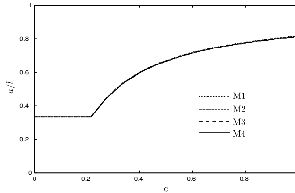
Figure 11. Crack growth with load c for the different meshes.
