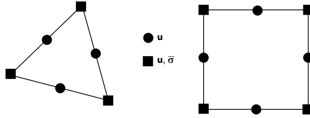
Figure 2. Nodal unknowns for two types of elements.
