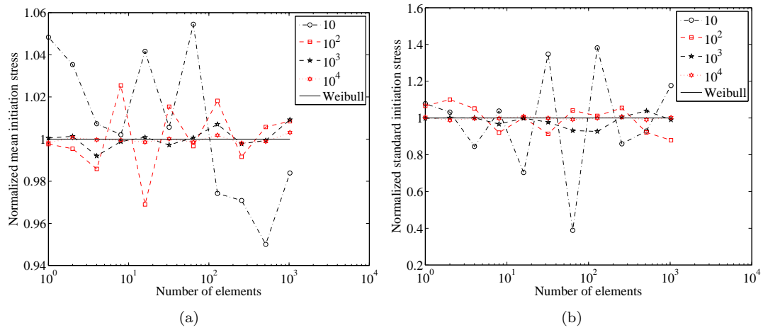
Figure 8. Normalized mean (a) and standard deviation (b) of the initiation stress as functions of the number of elements for the numerical model and the number of random selections. The straight solid line corresponds to initiations described by a Weibull model.
