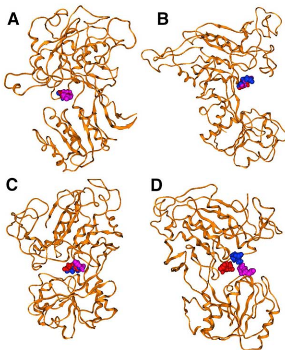
Figure 3: Glutamate diffuses away from the open site of Form 2, but not from other sites. Protein backbone is shown as an orange ribbon. Glutamate position at early, middle, and late time points in the simulation are shown as red, blue, and magenta spacefilling structures, respectively. A, Closed subunit of Form 1. B, Open subunit of form 1. C, Closed subunit of Form 2. D, Open subunit of Form 2.
