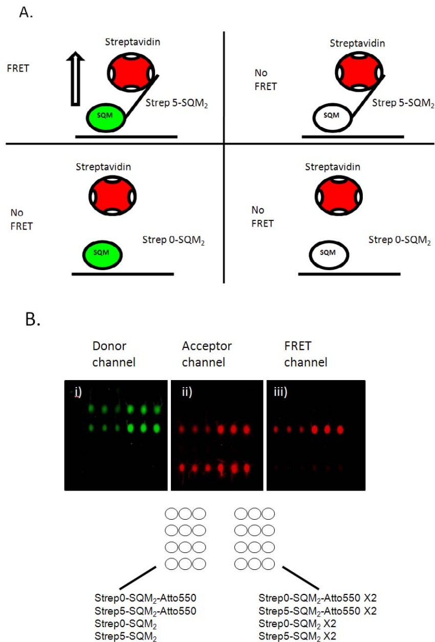
Fig. 5. A. Experiment and control scenarios which define the specificity of the FRET assay. FRET will only occur when both StrepX-SQM 2 and streptavidin are labelled with donor (green) and acceptor (red) dyes, and when the StrepX-SQM 2 is present to bring the donor and acceptor units together in proximity. StrepX-SQM 2 proteins are in the dimeric state. B) Microarray FRET assay measured in different emission channels. i)
