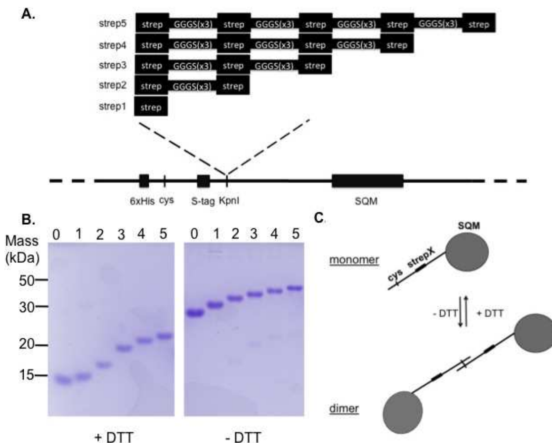
Fig. 1. A. Multiple cloning site region of the pET30a + -SQM construct used in this study. All streptavidin binding tags were inserted into the KpnI restriction site. Approximate location of the cysteine residue (cys) is indicated. B. Purified samples of StrepX-SQM separated on SDS-PAGE with and without DTT followed by staining with Coomassie blue. Dimer formation mediated by the cysteine residue is readily observed as a molecular weight shift (increase) in the oxidised state (-DTT). Numbers 1-5 signify number of Strep-tags (X) in the monomer. C. Schematic representation of dimer formation by StrepX-SQM.
