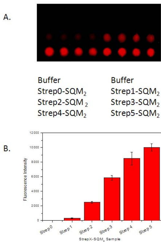
Fig. 4. A. Microarray spotting of StrepX-SQM 2 sample capture of Atto-647N labelled streptavidin. The microarray consists of seven spotted samples: a buffer control (spotted twice) and six StrepX-SQM 2 samples (X= 0-5). Each line contains two samples each, spotted in repeats of four. There are four lines in total, the first two lines cannot be seen due to no signal (buffer control, Strep0-SQM 2 ) or low signal (Strep1-SQM 2 ). B Relative average intensities with standard deviations over four samples of captured streptavidin emission.
