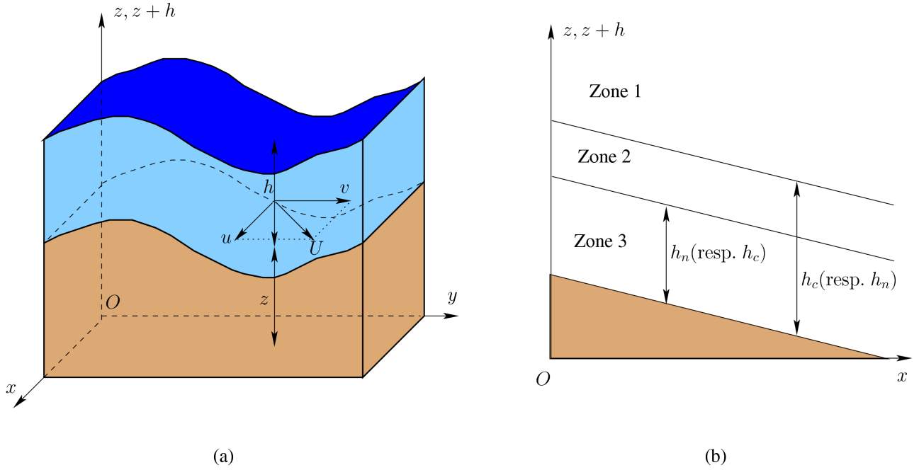
Figure 1: Illustration of variables of (a) Shallow Water equations and (b) zones for classification of free surface profiles.
