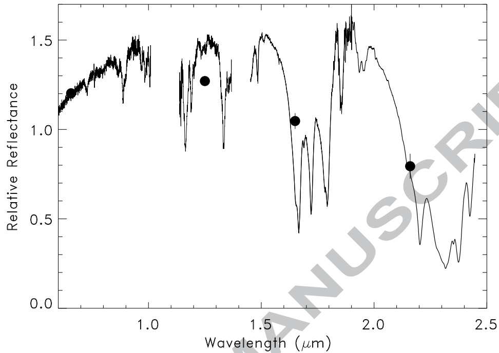
Fig. 6.— Reflectance spectrum of Pluto on the entire 0.6\text{-}2.5\mu\text{m} range obtained from the combination of the different spectra normalized at 1 in V band. The visible spectrum has been obtained during the first night and the near-IR spectra during the second night. Black points correspond to the reflectivity obtained in each photometric band (see text for more details).
