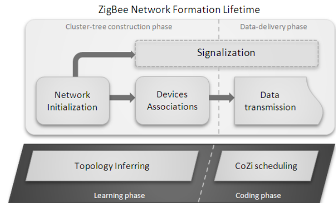
Fig. 2 – CoZi architecture overview
