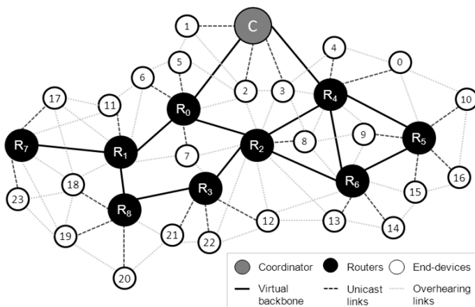
Fig. 1 – ZigBee network topology illustration
