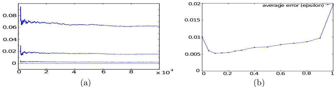
FIGURE 4. (a): Evolution of the ring bounds; (b): Averaged error of AEE as a function of \epsilon .
